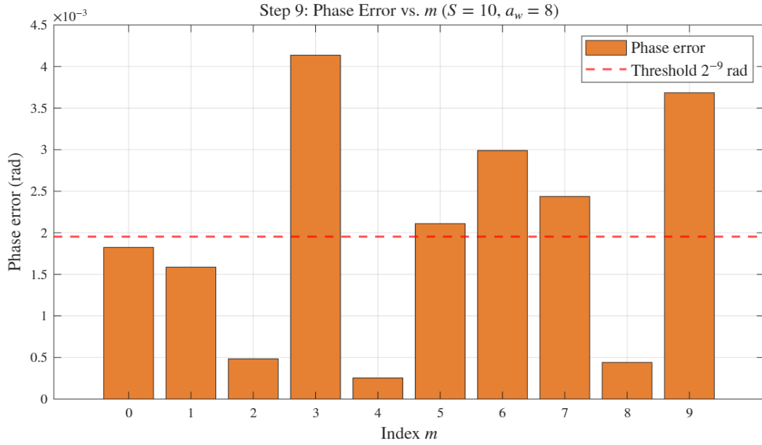
Figure 17: Step 9: Phase error for all 10 test inputs. All mismatches = 0.
