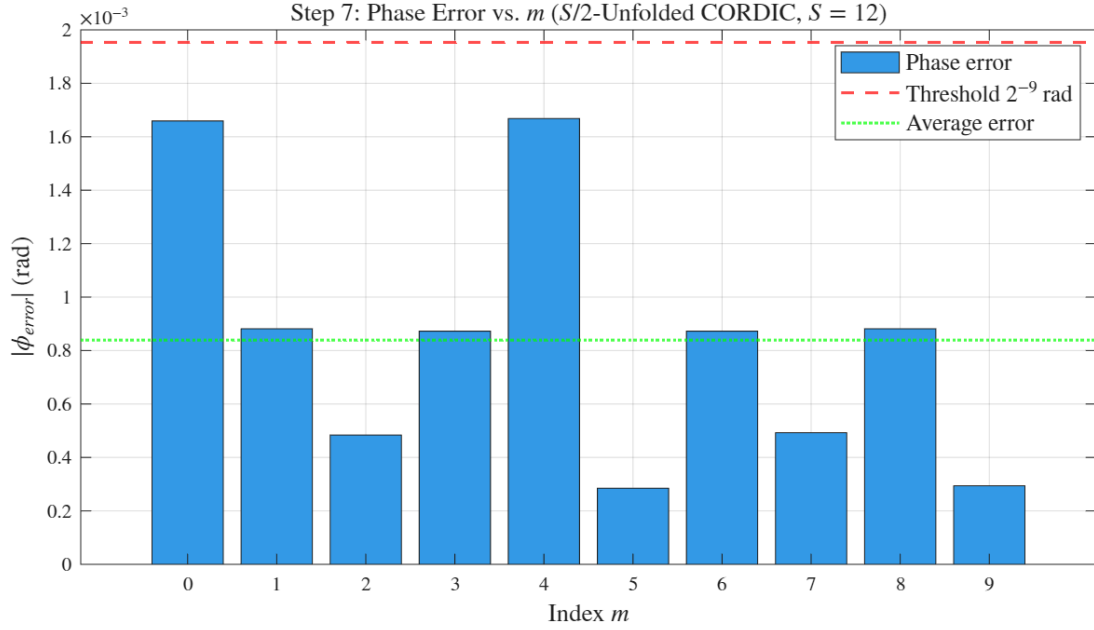
Figure 15: Step 7: Phase error between post-synthesis simulation results and floating-point arctangent reference ( m = 0, \dots, 9 ). Results are identical to behavioral simulation, confirming bit-exact agreement after synthesis.
