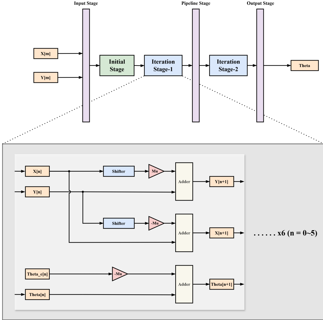
Figure 11: S/2-Unfolded CORDIC architecture: top-level pipeline (Input \rightarrow Stage-1 \rightarrow Pipeline FF \rightarrow Stage-2 \rightarrow Output) and expanded single-iteration datapath ( \times 6 , n = 0 \dots 5 ).
