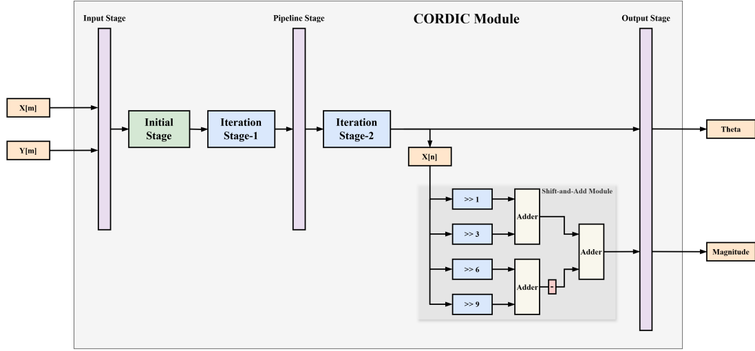
Figure 16: Full CORDIC Module architecture: Input Stage, Initial Stage, Iteration Stage-1, Pipeline Stage, Iteration Stage-2, CSD Shift-and-Add, and Output Stage producing both Theta and Magnitude.
