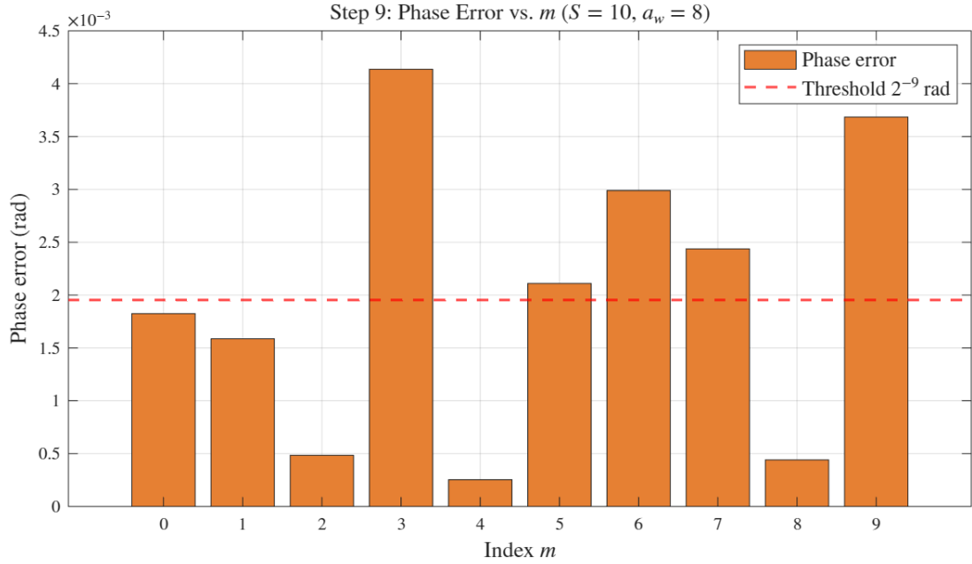
Figure 21: Step 9: Phase error between post-synthesis simulation results and floating-point arctangent reference ( m = 0, \dots, 9 ). Results are identical to behavioral simulation, confirming bit-exact agreement after synthesis.
