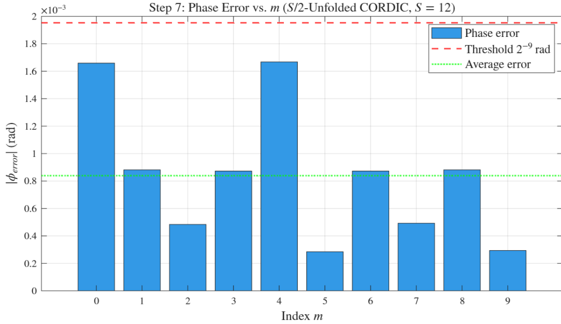
Figure 12: Step 7: Phase error for all 10 test inputs. All mismatches = 0 confirms bit-exact match.
