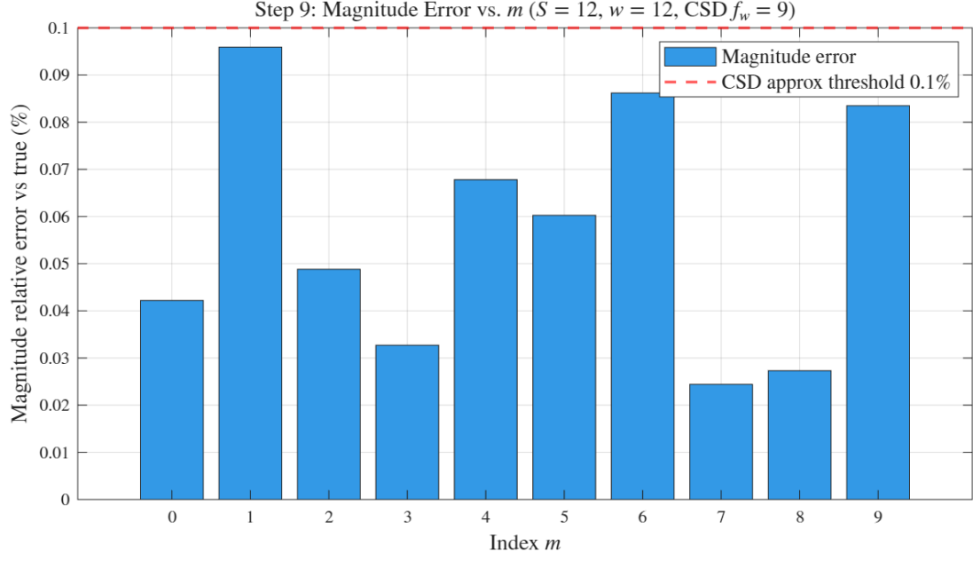
Figure 22: Step 9: Magnitude error (%) between post-synthesis simulation results and true magnitude ( m = 0, \dots, 9 ). Maximum error < 0.1\% , consistent with the CSD approximation bound.
