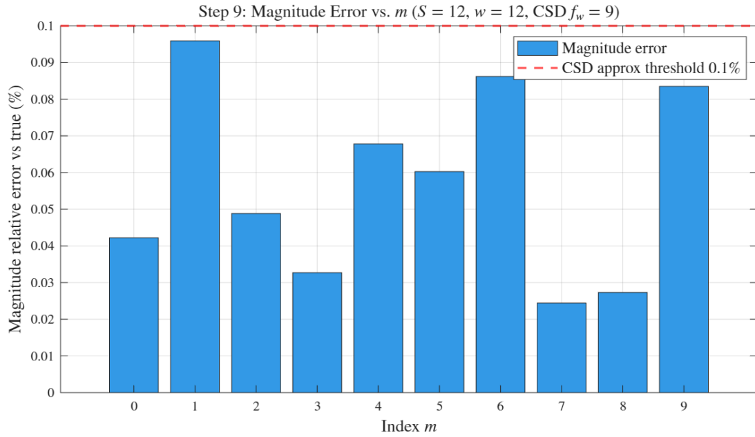
Figure 18: Step 9: Magnitude error (%) for all 10 test inputs. Maximum error < 0.1\% , consistent with the CSD approximation bound.
