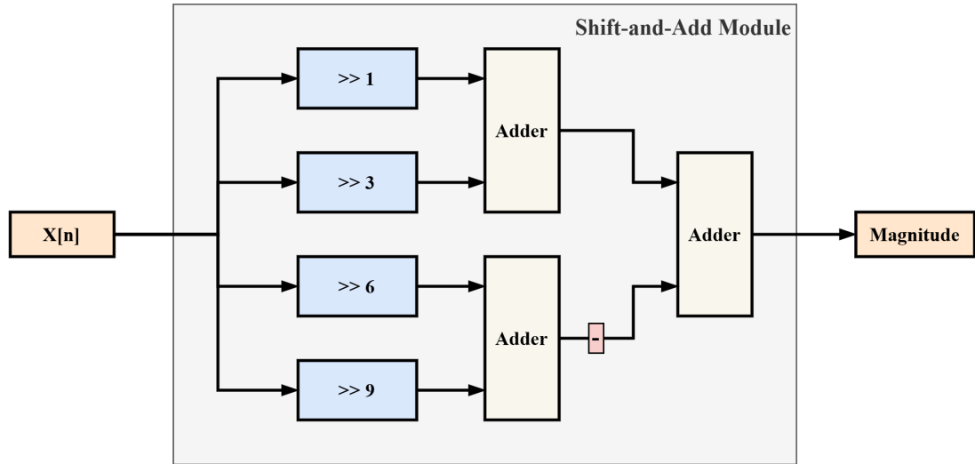
Figure 7: CSD Shift-and-Add Module: A_N = 2^{-1} + 2^{-3} - 2^{-6} - 2^{-9} , implemented with 3 adders.
