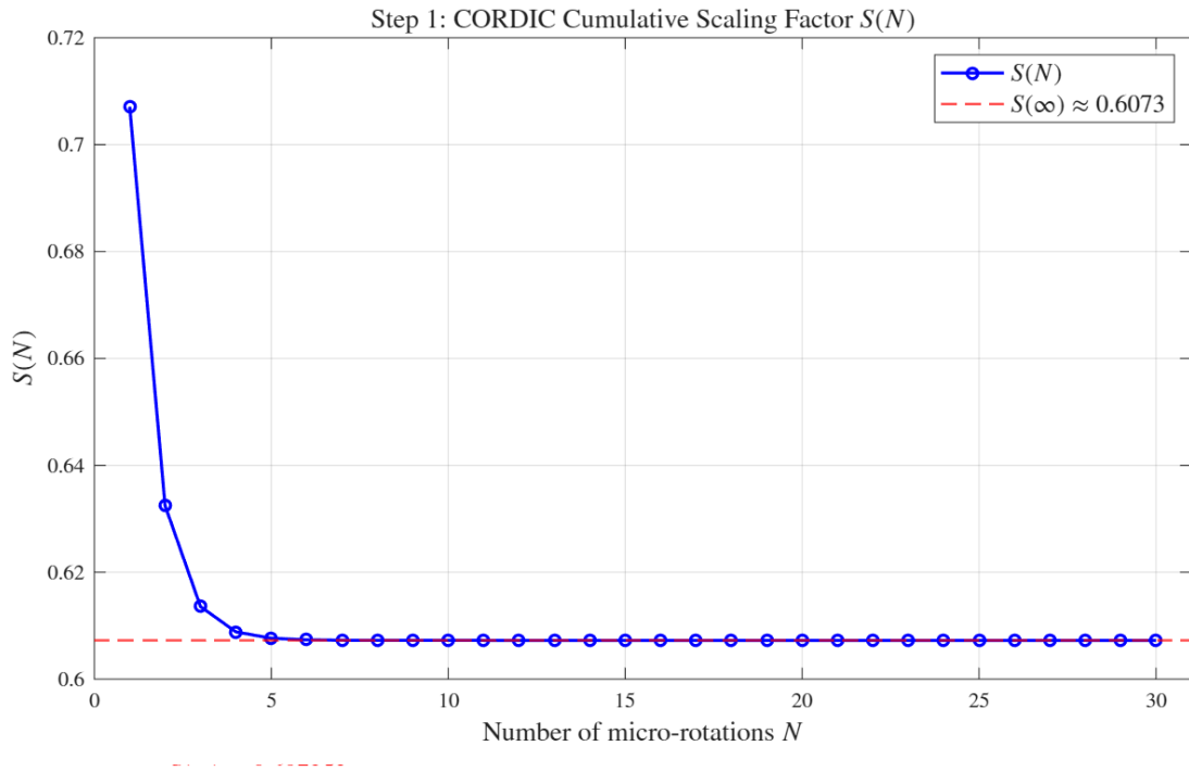
Figure 1: S(N) vs. N . The curve saturates rapidly; the converged value is S(\infty) \approx 0.607253 .
