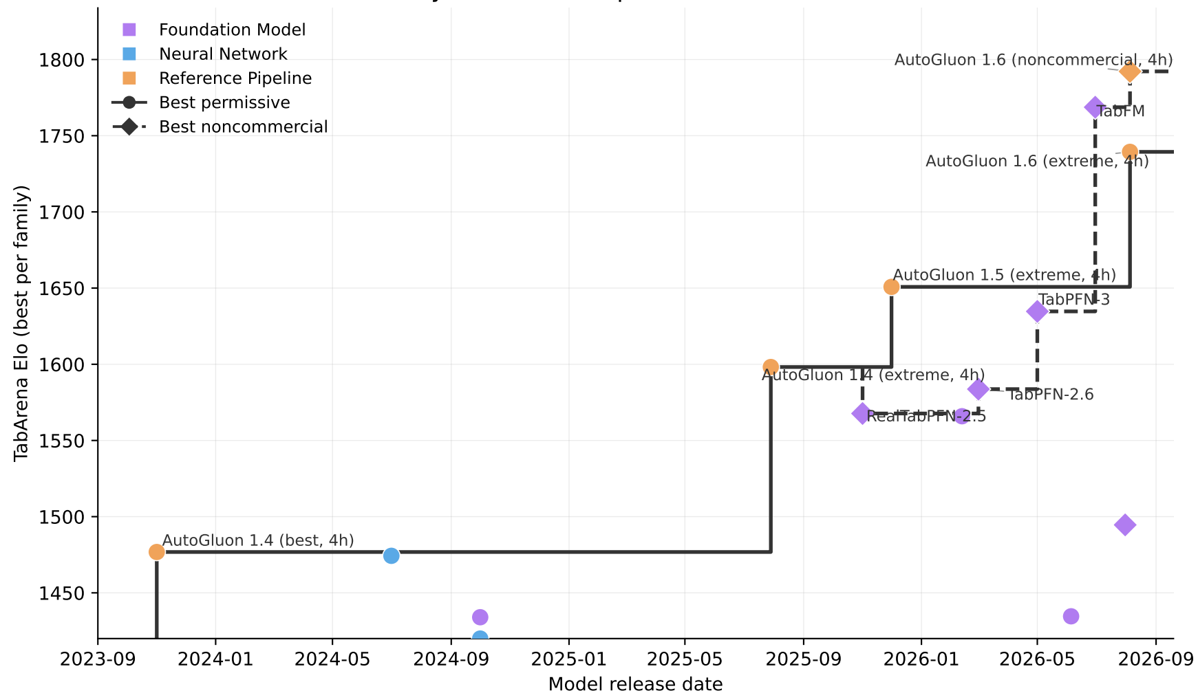
Tabular model Elo by release date: permissive vs noncommercial licenses
