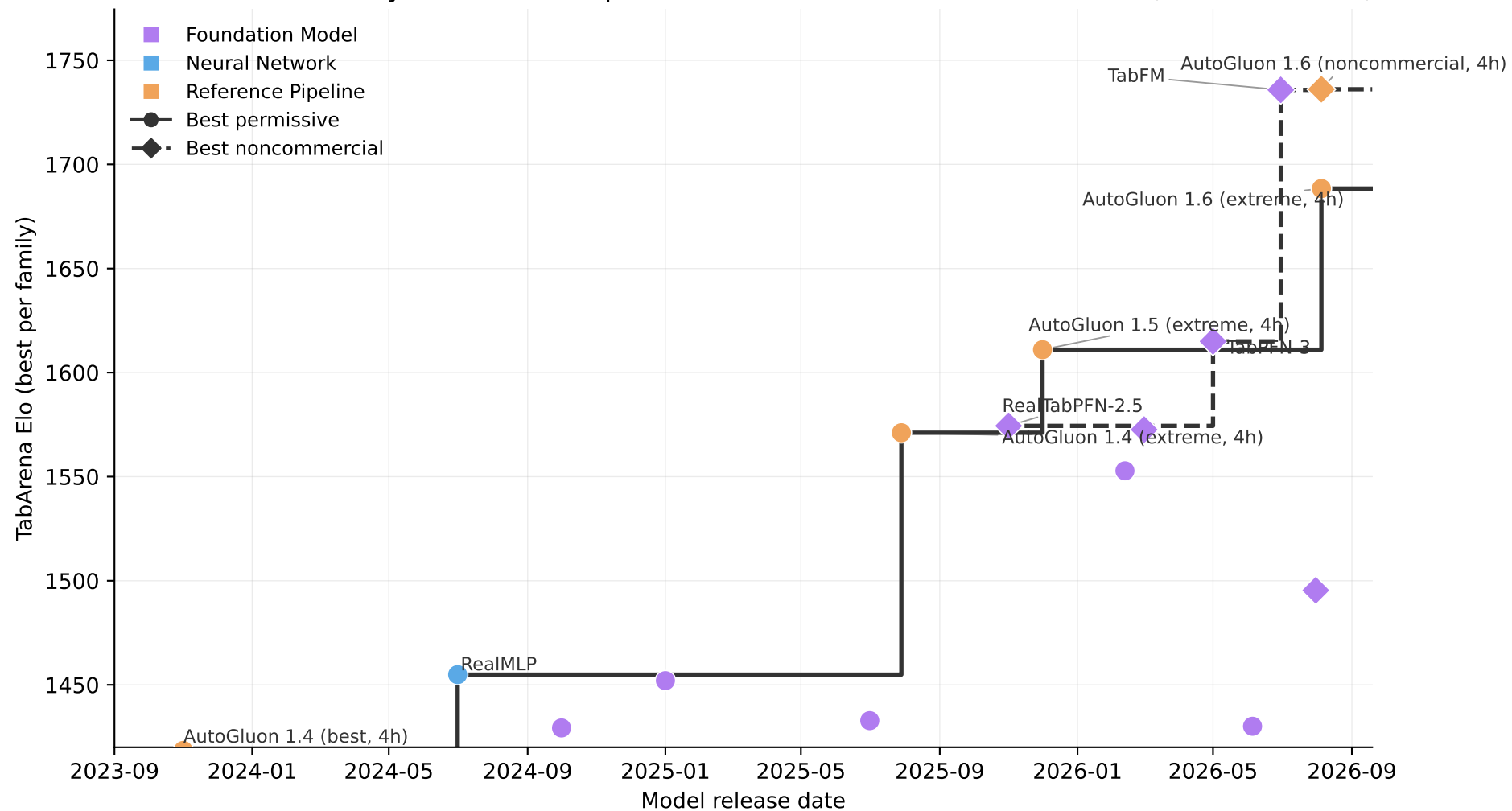
Tabular model Elo by release date: permissive vs noncommercial licenses (small datasets)
