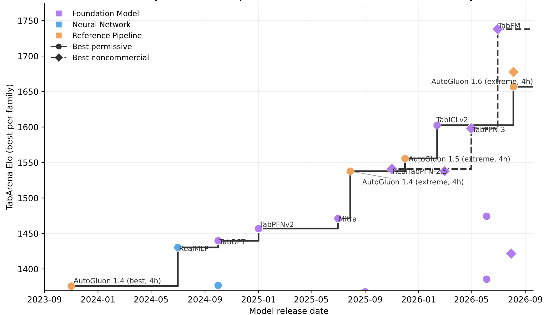
Tabular model Elo by release date: permissive vs noncommercial licenses (tiny datasets)
