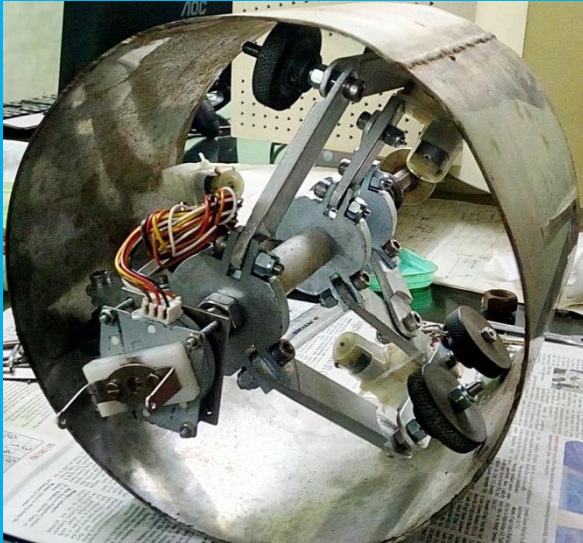
Sewage Pipe Robot
