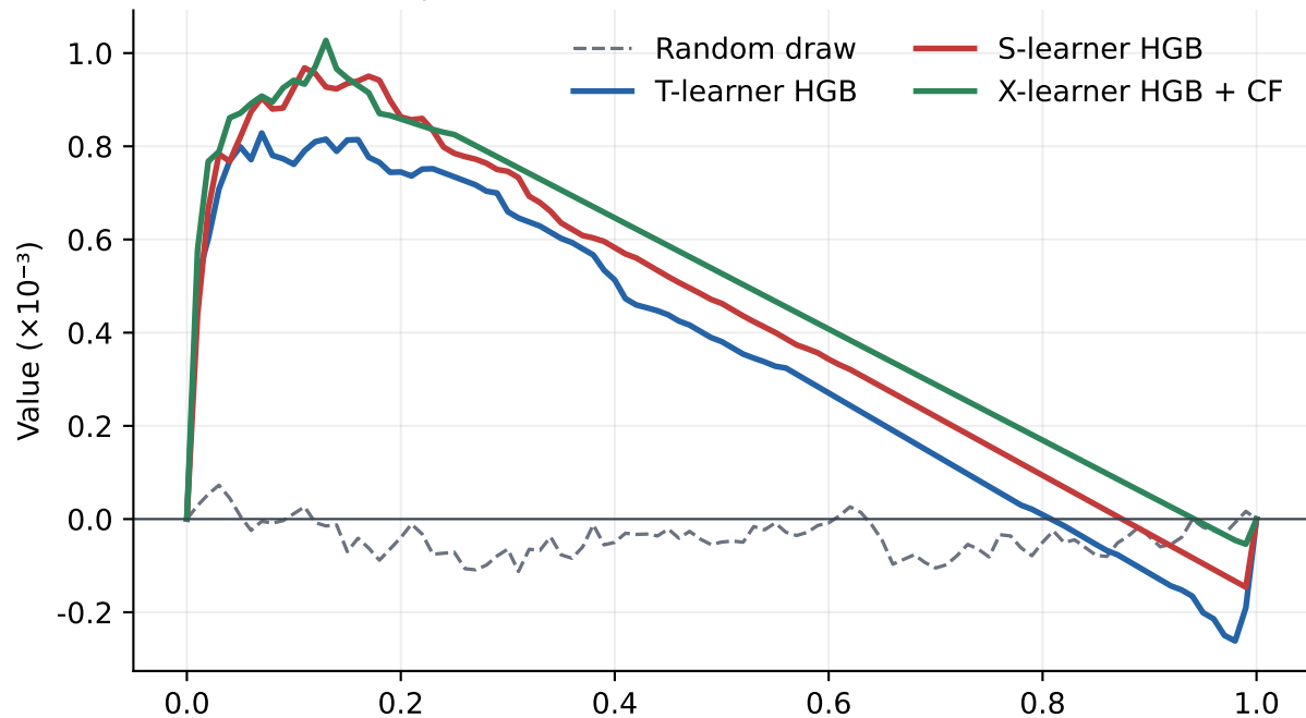
Development validation Qini curves (seed 2027)
