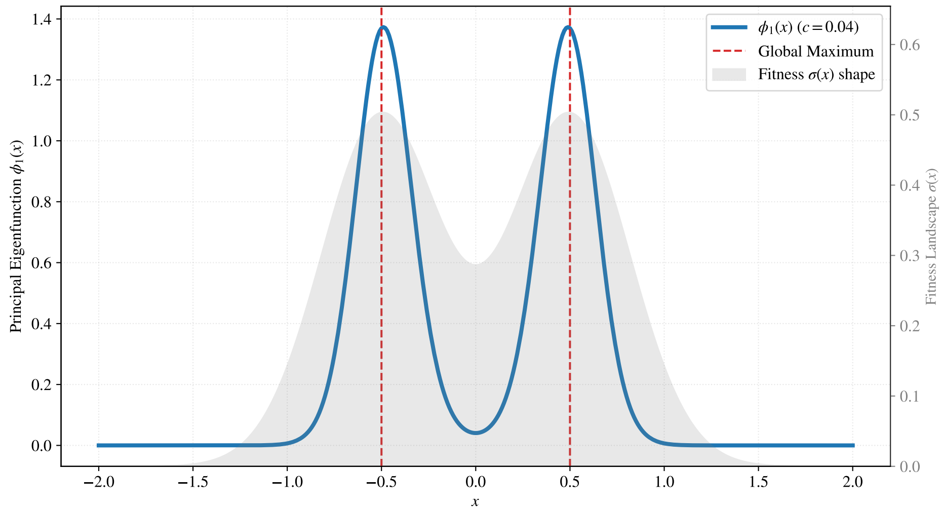
Concentration of \phi_1 for fixed c = 0.04
