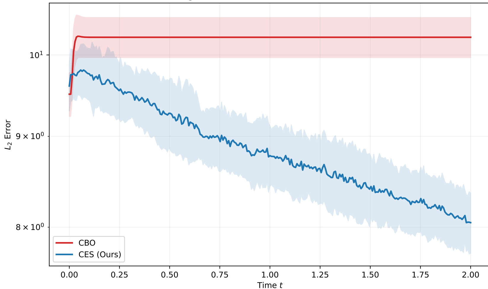
Convergence Profile (d=30, Shifted Initialization)
