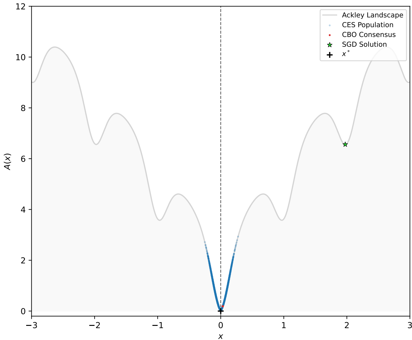
Final Solutions: 1D Ackley
