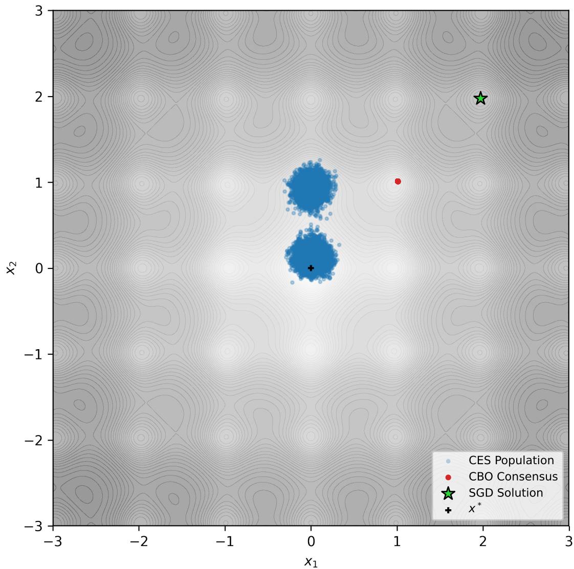
Final Solutions: 2D Ackley
