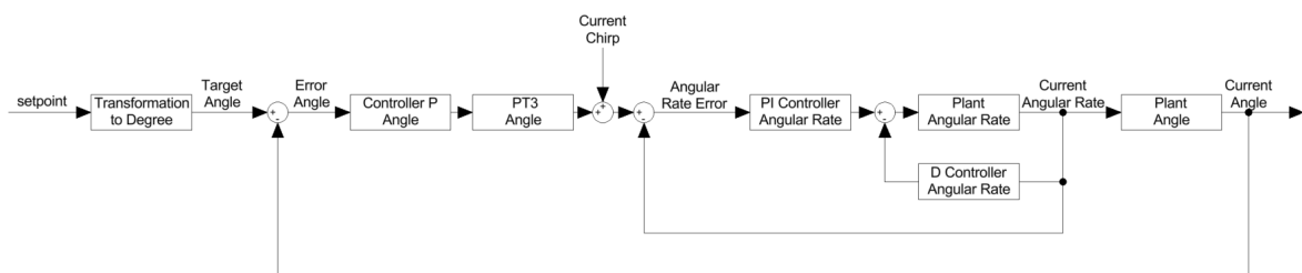
Figure 3.5: Cascaded control structure of the Betaflight Angle mode controller.
