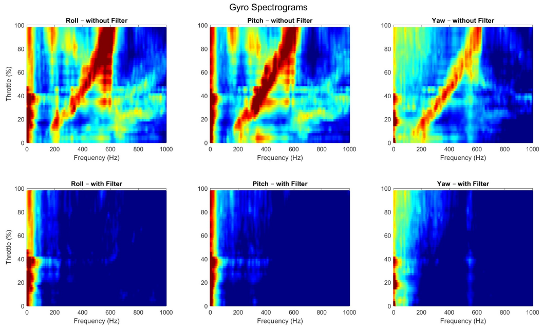
Figure 3.2: Spectrograms
