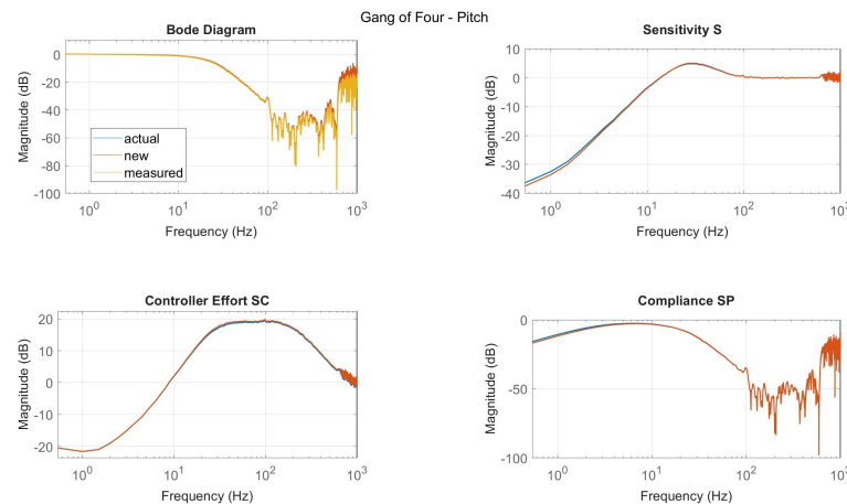
Figure 3.4: Gang of Four
