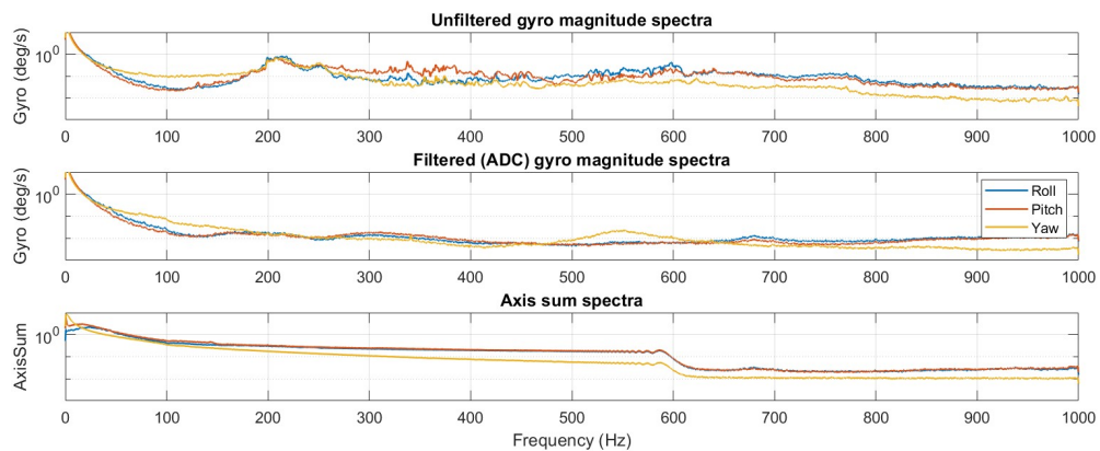
Figure 3.1: Spectra
