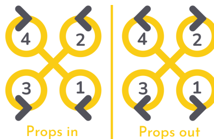
Figure 2.3: Propeller rotation directions for a quadcopter in “props in” and “props out” configuration.
