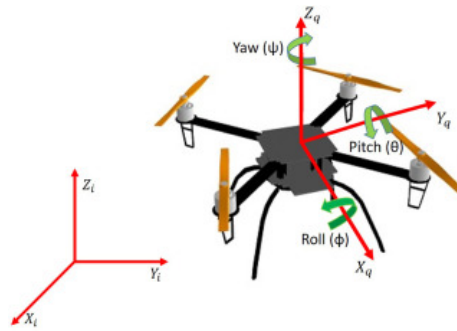
Figure 2.2: Body-fixed coordinate system and rotational axes of a quadcopter.
