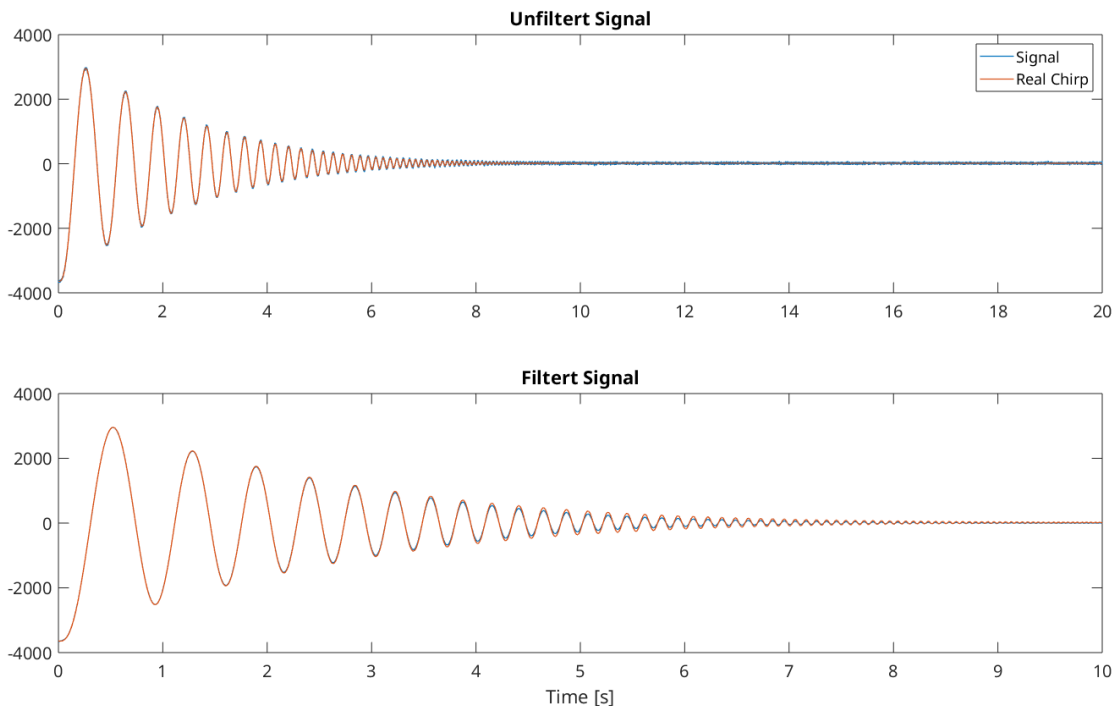
Figure 2.7: Time-domain signal before (top) and after (bottom) baseband filtering.
