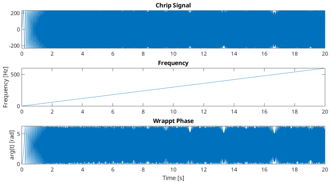
Figure 2.3: Linear chirp signal used for the simulation.
