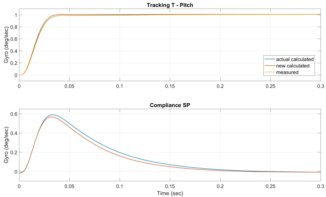
Figure 3.4: Step Response
