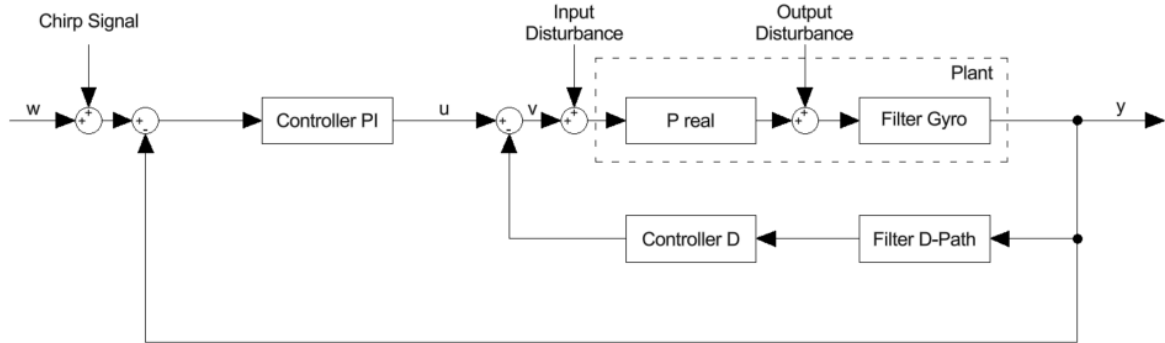
Figure 3.1: Control loop structure in Acro mode
