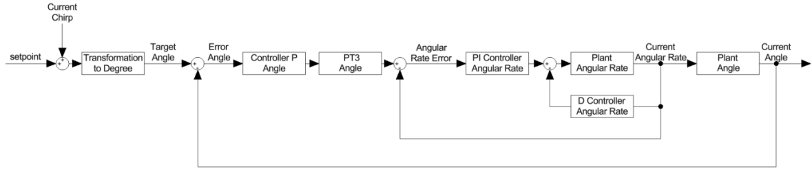
Figure 3.7: Cascaded control structure of the Betaflight Angle mode controller.
