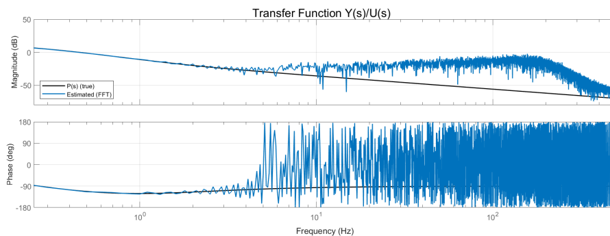
Abbildung 8: Bode plot estimated with plain FFT
