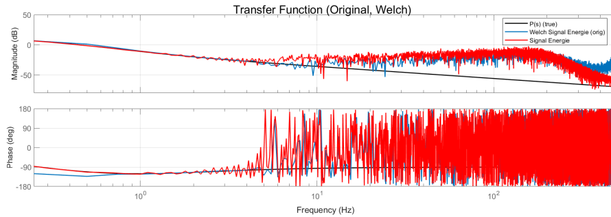
Abbildung 9: Bode plot estimated with Welch method
