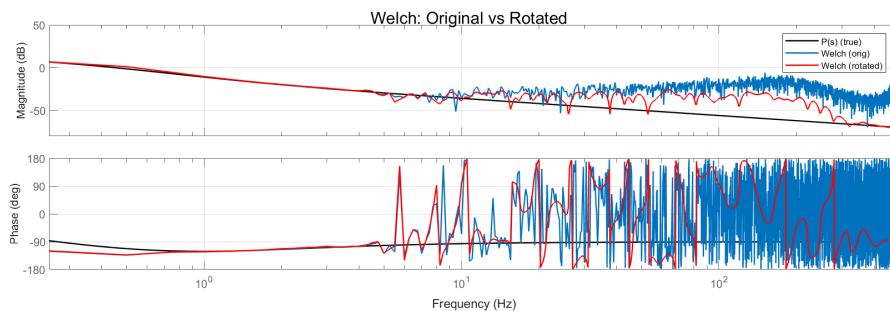
Abbildung 10: Bode plot estimated with rotated Welch method
