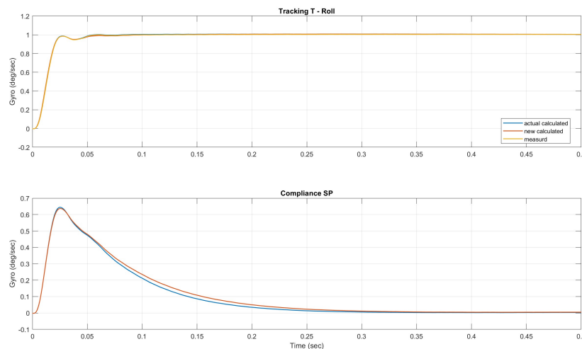
Abbildung 14: Step Response
