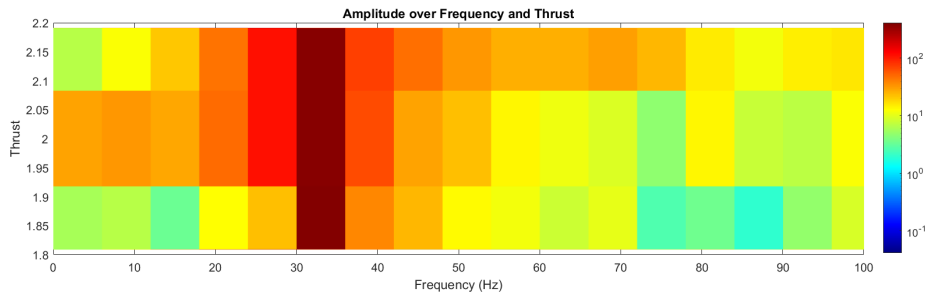
Abbildung 12: Spectrogram over thrust
