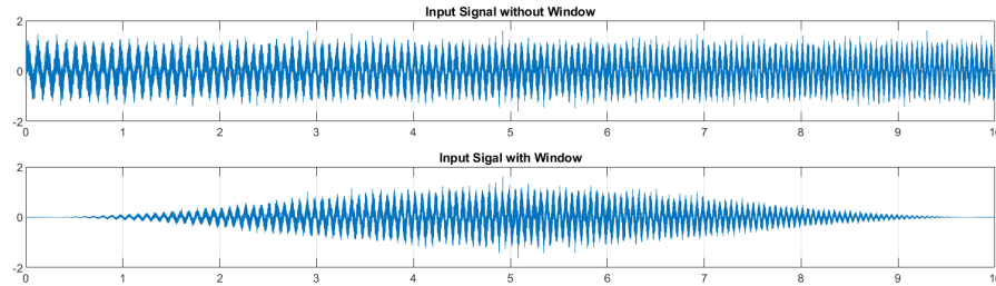
Abbildung 6: Comparison of Signal with and without windowing
