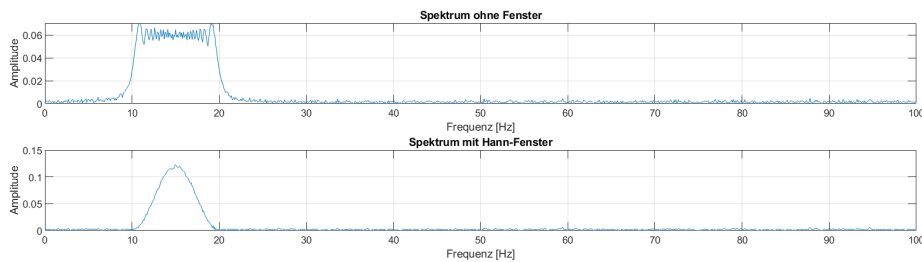
Abbildung 7: Comparison of Spectra with and without windowing
