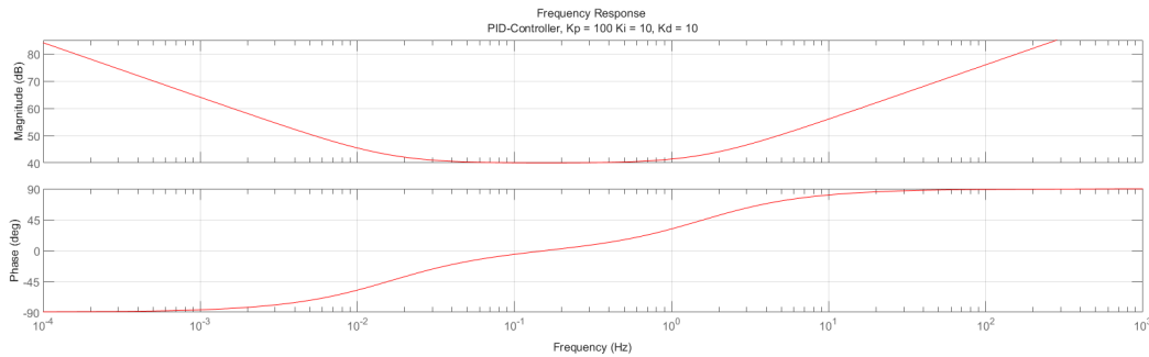
Abbildung 5: Bodeplot out of Controller Simulation
