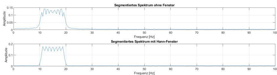
Abbildung 8: Comparison of Spectra with and without windowing
