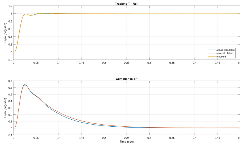
Abbildung 10: Step Response
