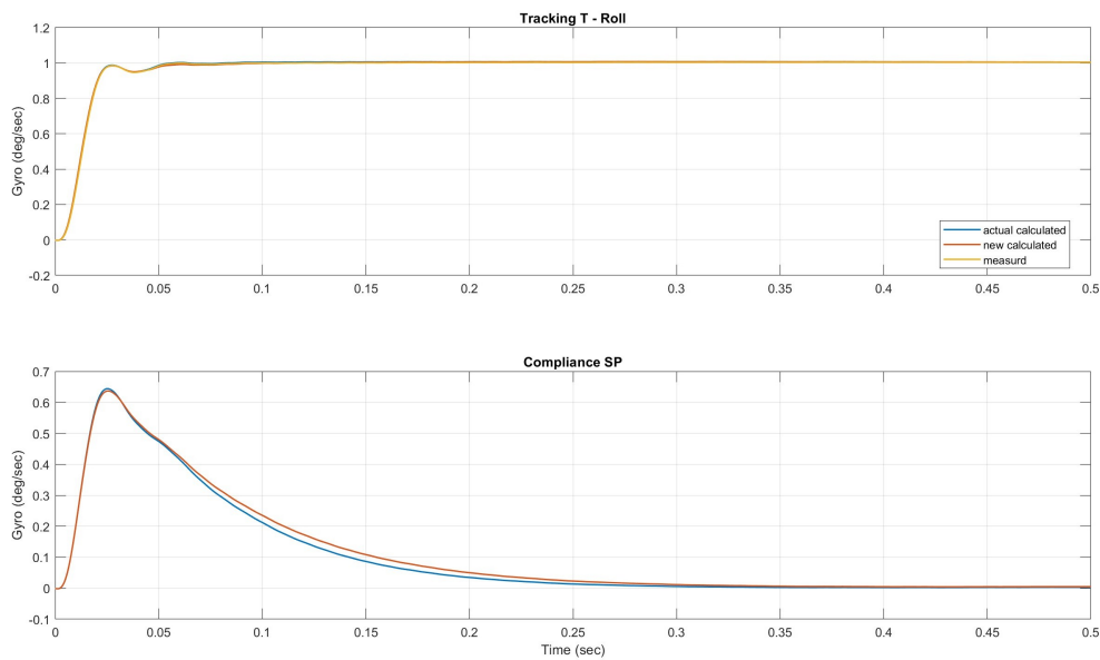
Figure 24: Step Response
