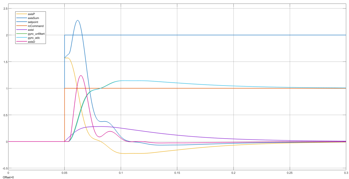
Figure 8: Simulated step response
