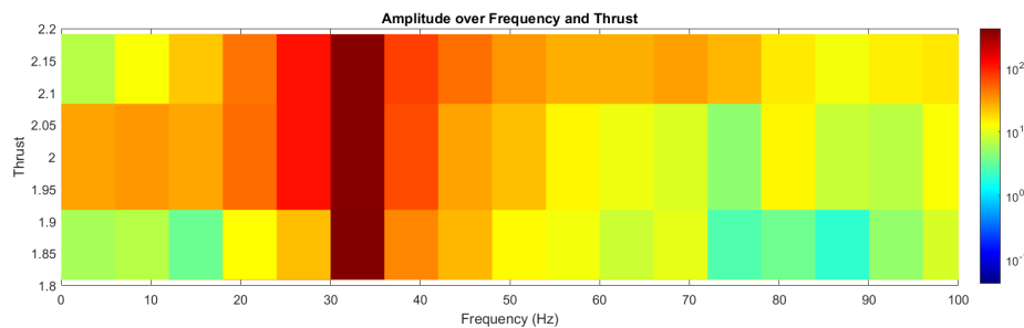
Figure 20: Spectrogram showing the amplitude over frequency and thrust.
