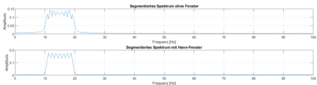
Figure 17: Spectrum with segment averaging
