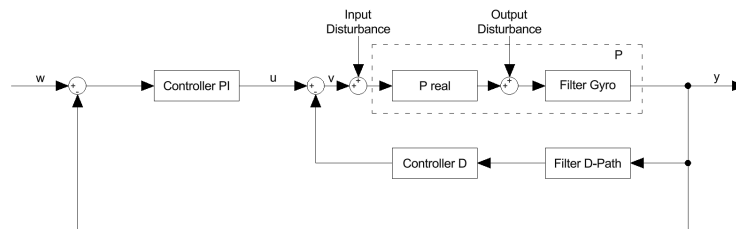
Figure 4: Gyro Control Loop
