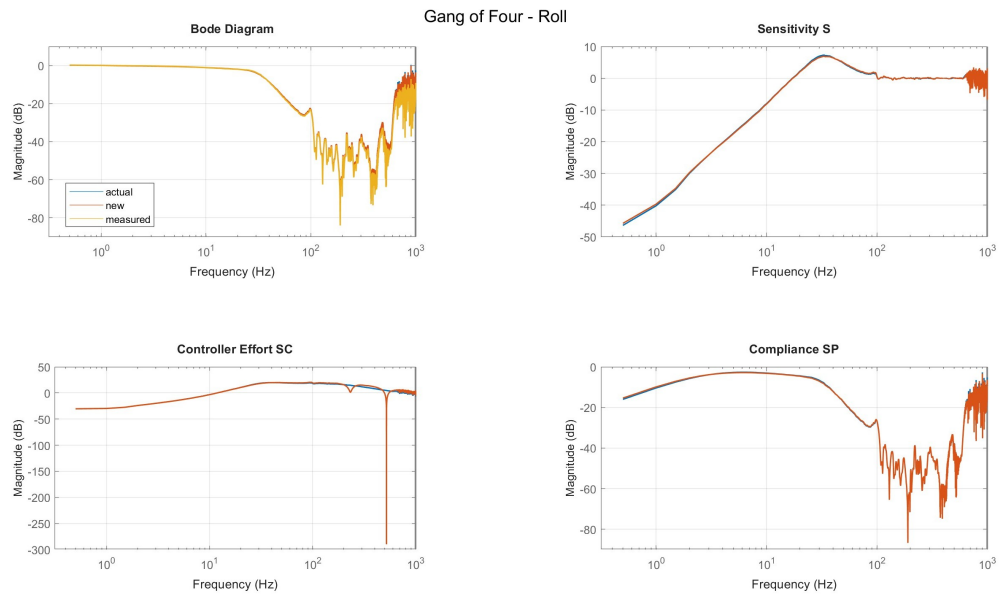
Figure 25: Gang of four
