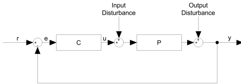
Figure 3: Simplified closed loop system
