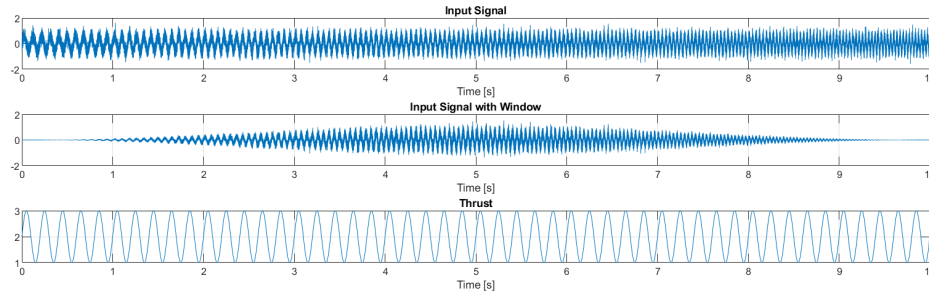
Figure 18: Input signal, windowed input signal, and thrust over time.
