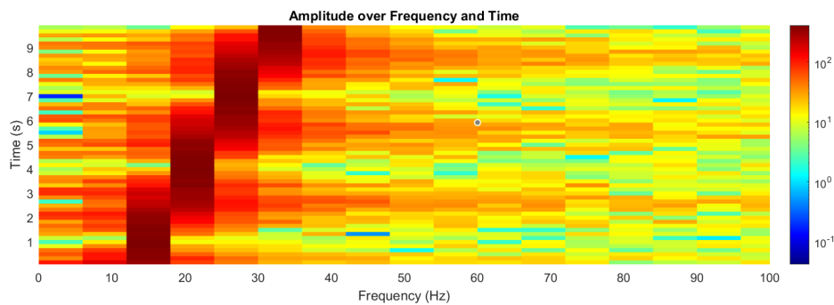
Figure 19: Spectrogram showing the amplitude over frequency and time.
