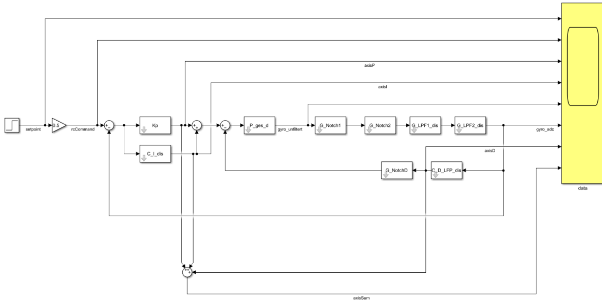
Figure 7: Simulink model of the Betaflight control system
