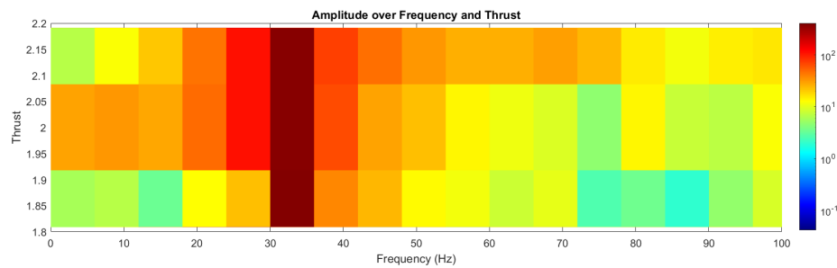
Abbildung 11: Spectrogram showing the amplitude over frequency and thrust.
