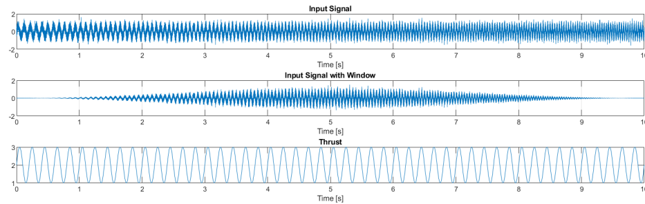
Abbildung 9: Input signal, windowed input signal, and thrust over time.
