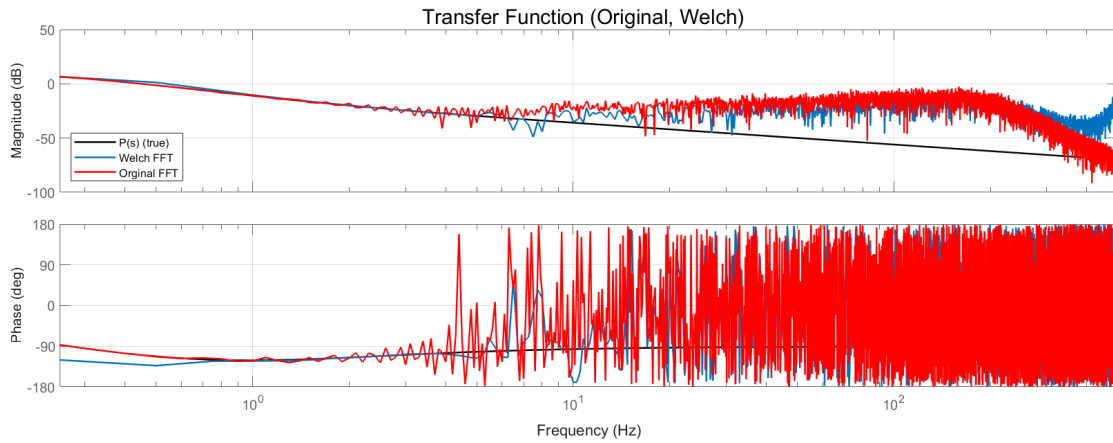
Abbildung 9: Bode plot estimated with Welch method
