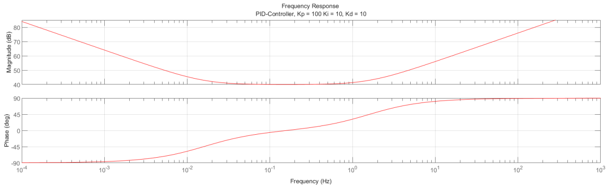
Abbildung 5: Bodeplot out of Controller Simulation
