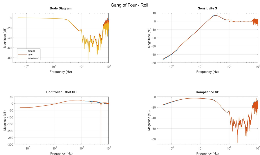
Abbildung 21: Gang of four
