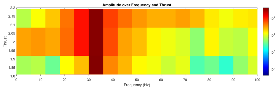
Abbildung 16: Spectrogram showing the amplitude over frequency and thrust.
