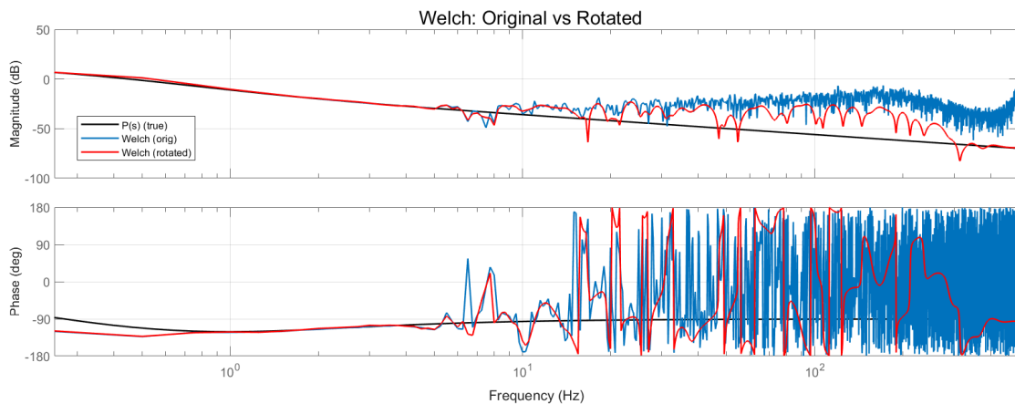
Abbildung 10: Bode plot estimated with rotated Welch method
