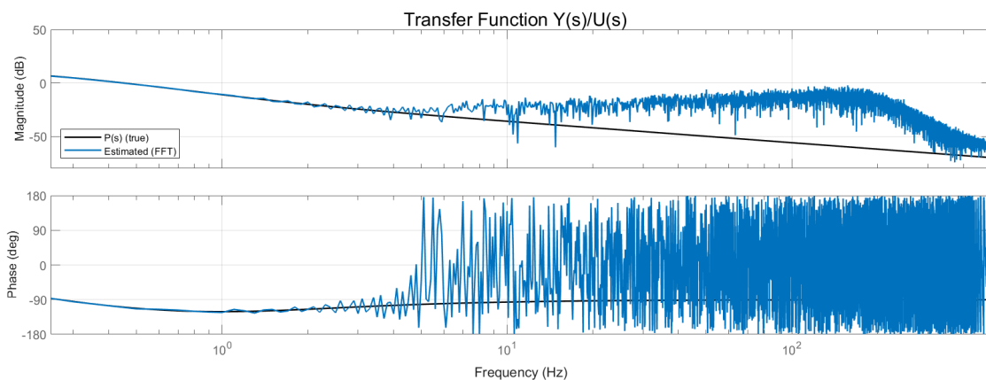
Abbildung 8: Bode plot estimated with plain FFT
