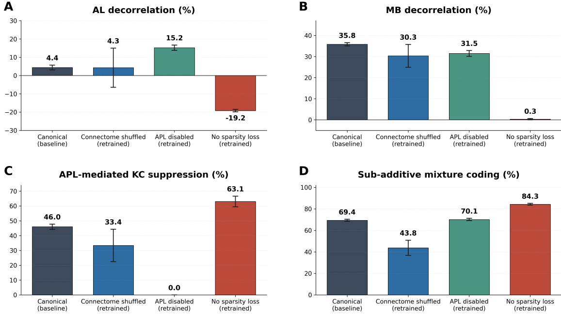
Figure 4: Circuit-component perturbations clarify each architectural feature’s contribution, comparing the canonical model against three retrained conditions: shuffled connectome, APL-disabled, and no-sparsity-loss (five-seed mean \pm 1 s.d.). (A) AL decorrelation rises sharply when the APL is removed, indicating that the APL maintains MB-localized decorrelation. Shuffling the connectome instead makes AL decorrelation highly variable—demonstrating that specific topology beyond degree distribution stabilizes and minimizes AL decorrelation—while removing the sparsity loss drives it strongly negative. (B) MB decorrelation is mostly preserved (although still less localized overall) under APL ablation. The shuffled connectome is again less stable than the canonical model for MB decorrelation, which collapses entirely without the sparsity loss. (C) The APL-mediated KC suppression of \sim 50\% reported by Mancini et al. (2023) falls to 0% when the APL is removed (confirming the ablation), is reduced and destabilized by shuffling the connectome, and is inflated in the densely ( \sim 80\% ) active KC regime without the sparsity loss. (D) Sub-additive mixture coding of \sim 73\% is reported by Honegger et al. (2011). The fraction of KCs whose 2-odor mixture response falls below the sum of their single-odor responses is unchanged by APL ablation, indicating it arises from other circuit components. It drops and is destabilized when the connectome is shuffled (again demonstrating the importance of connectome topology) and rises in the dense no-sparsity regime.
