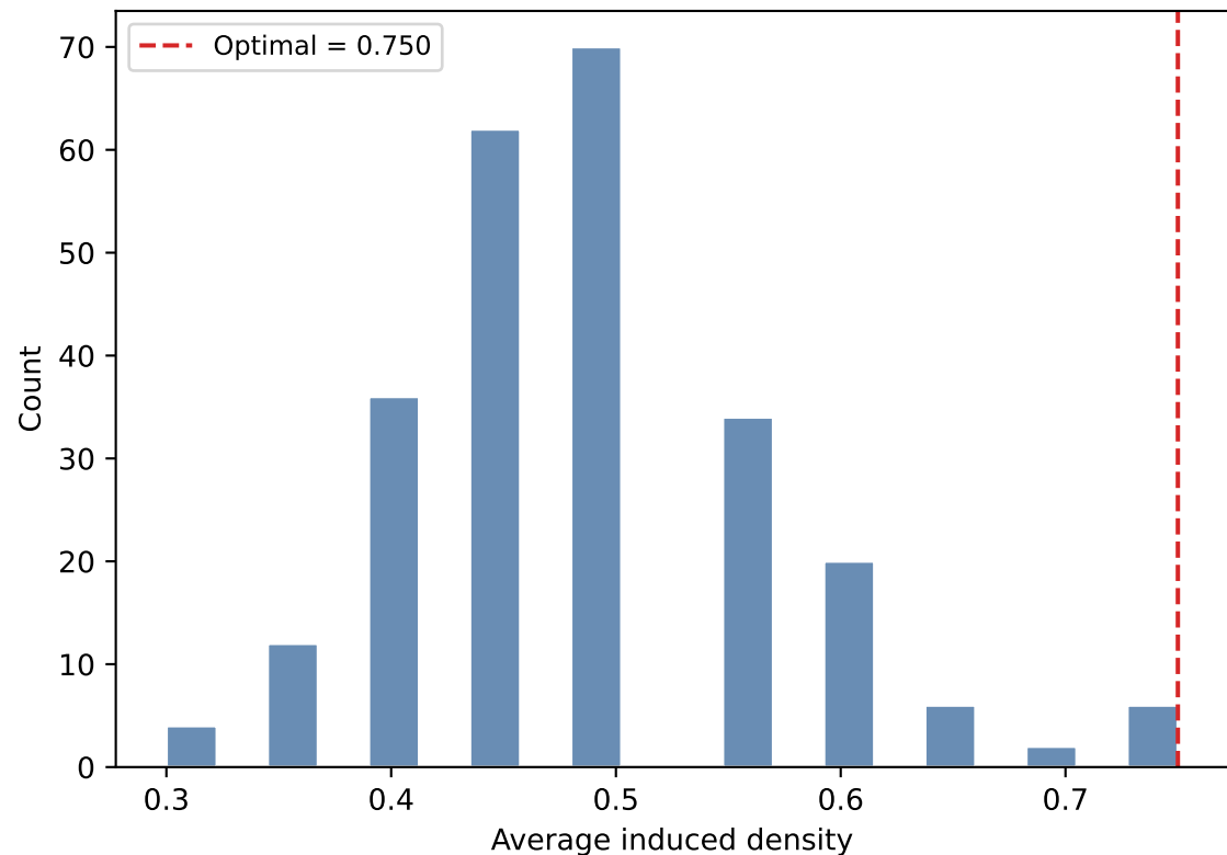
Distribution of Bisection Densities Optimal: keter | chokhmah | binah | chesed | gevurah vs tiferet | netzach | hod | yesod | malkhut
