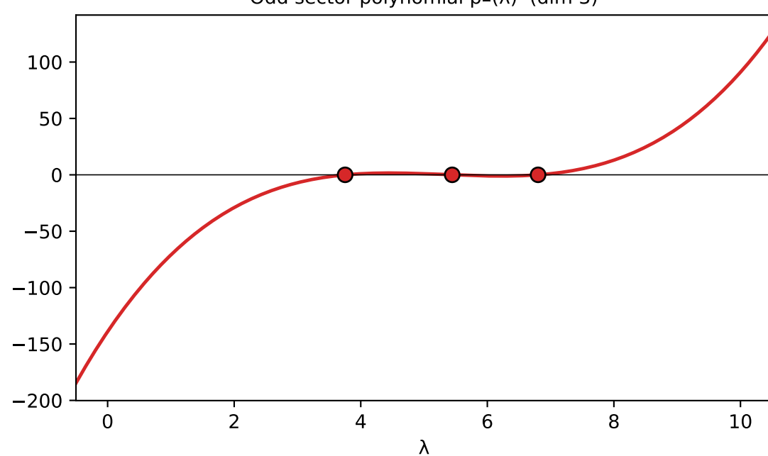
Odd sector polynomial p_-(\lambda) (dim 3)
