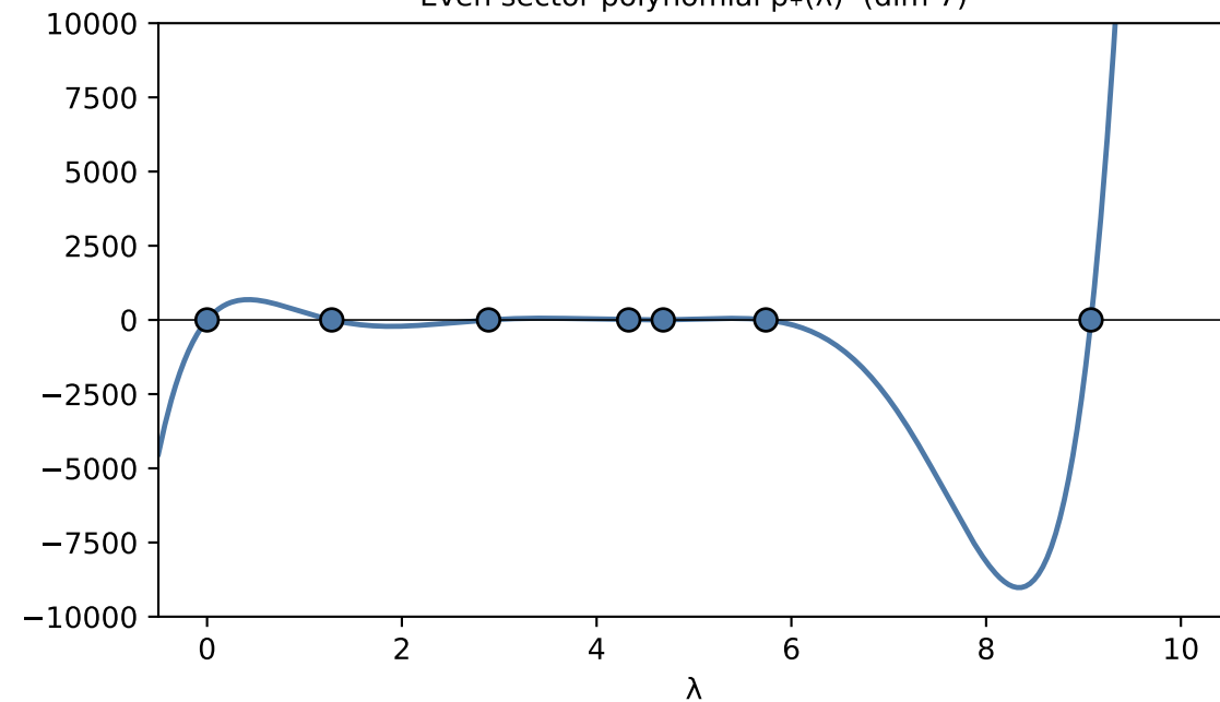
Even sector polynomial p_+(\lambda) (dim 7)
