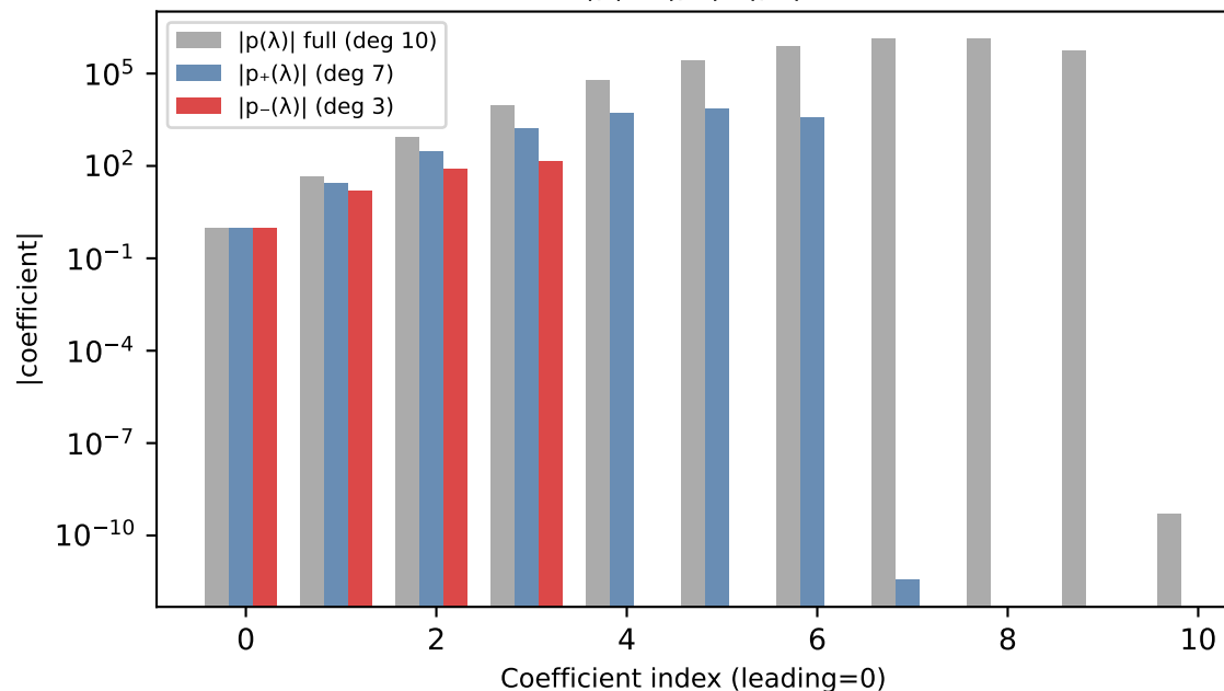
Odd sector polynomial p_-(\lambda) (dim 3)
