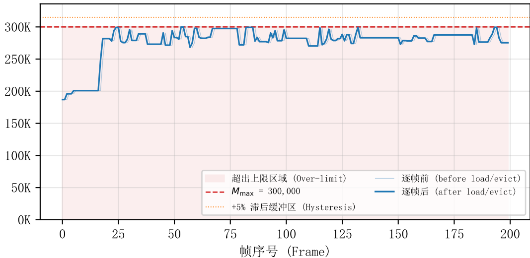
GPU锚点数量稳定性 (GPU Anchor Count Stability)
