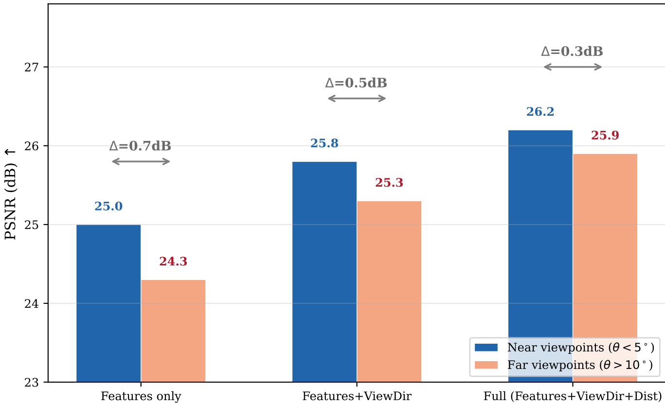
Viewpoint Robustness: PSNR Across Viewing Angles
