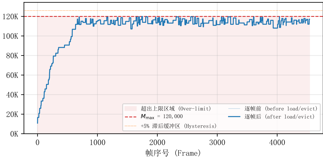
GPU锚点数量稳定性 — KITTI seq00 (GPU Anchor Count Stability)
