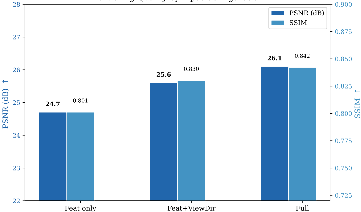
Rendering Quality by Input Configuration
