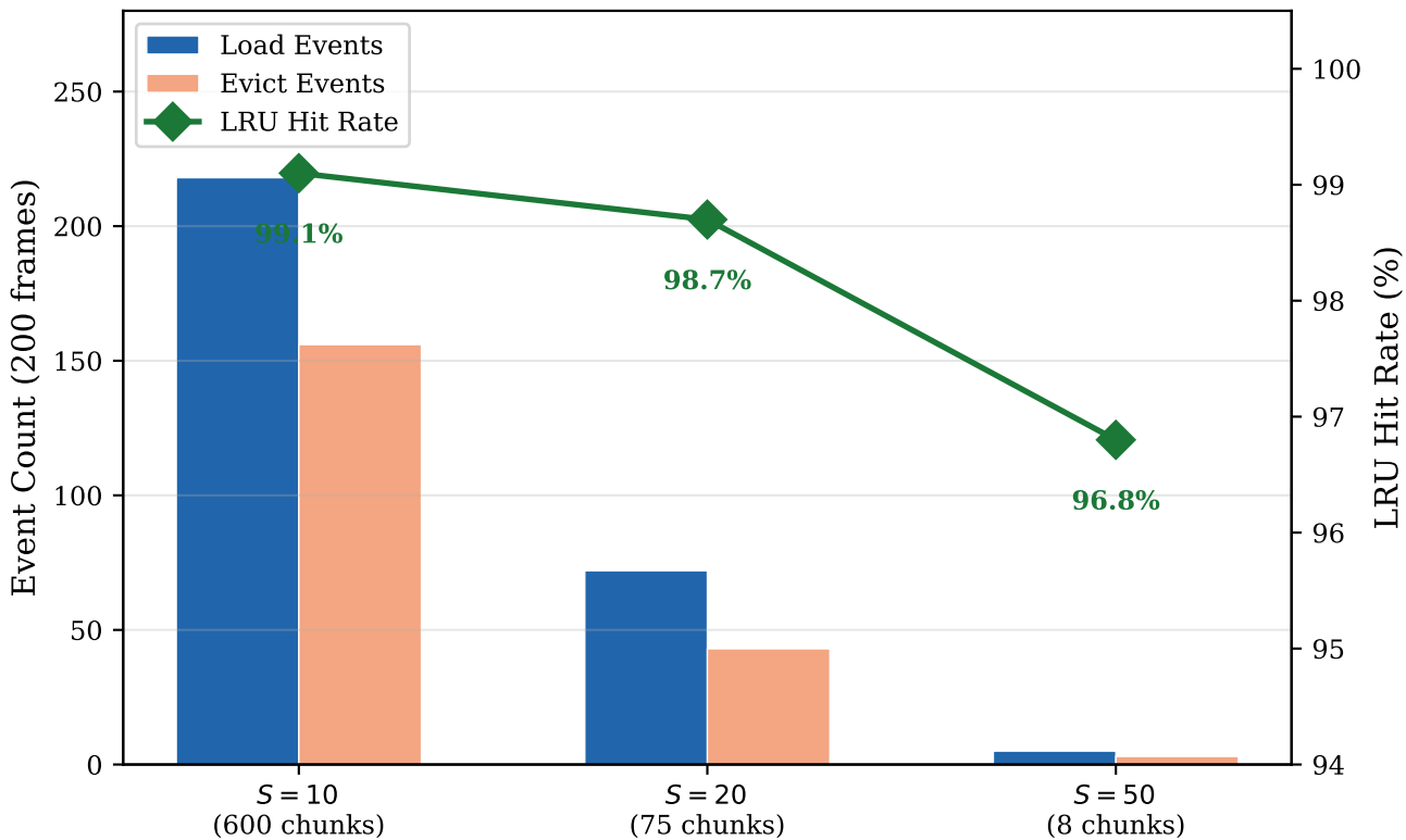
Chunk Size Ablation: I/O Events & Hit Rate
