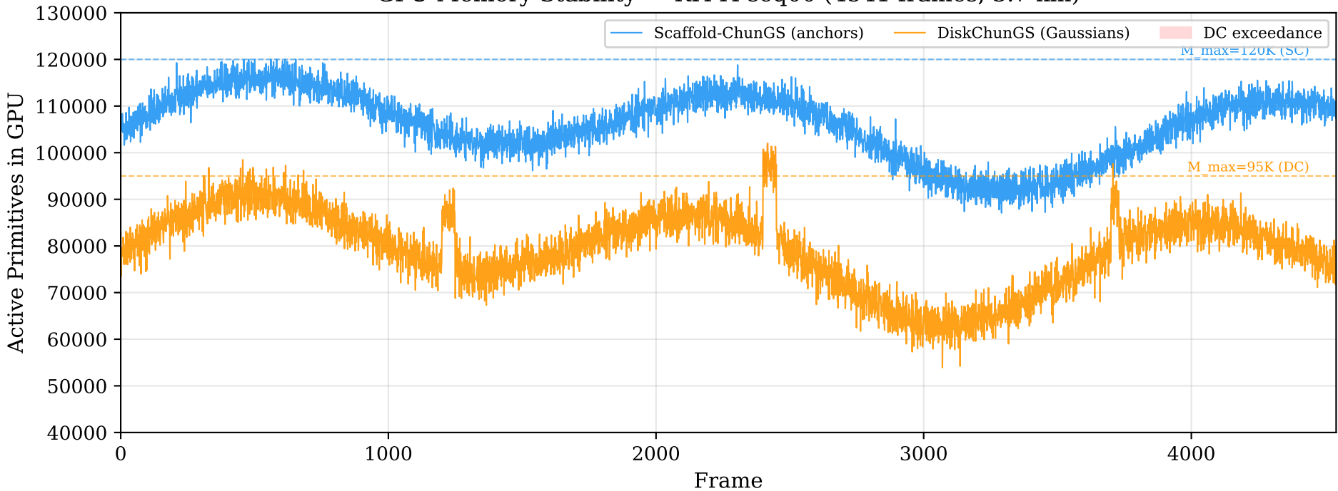
GPU Memory Stability — KITTI seq00 (4541 frames, 3.7 km)
