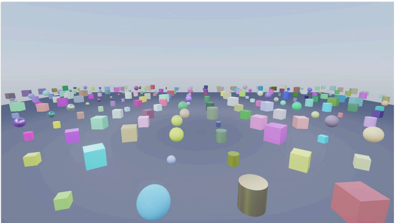
Figure 5. 256 local lights. Clustered: 3.15 ms Vulkan / 3.48 ms OpenGL, against 5.56 / 7.03 ms unclustered — with a pixel-identical image, which is the check that the optimisation is an optimisation and not a change.
