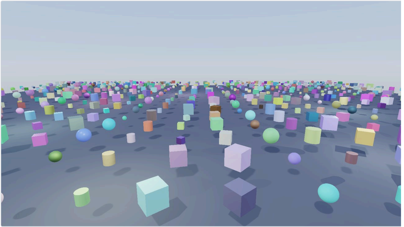
Figure 4. The stress scene — 1000 meshes at 1.88 ms (Vulkan) and 1.59 ms (OpenGL), Release, vsync off. OpenGL winning here is real and not a bug: at this draw count the frame is dominated by per-draw CPU cost, where GL's simpler binding model has less to do.
