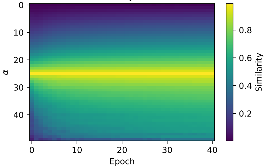
Model Similarity Over Time
