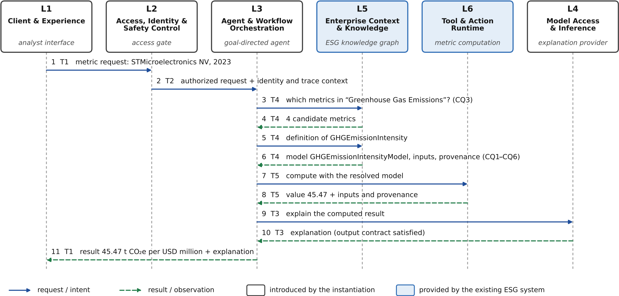
11 recorded interaction occurrences realizing 5 of 8 interaction types. L2 applies its egress check to the result before L1 presents it.
