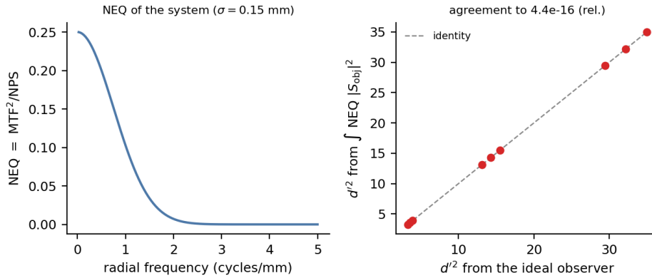
Figure 2. The physical-to-task bridge. Left: the NEQ = MTF^2/NPS of the system. Right: d'^2 computed from the ideal observer (horizontal) against d'^2 computed by integrating NEQ against the object power spectrum (vertical), for nine contrast-by-blur conditions; the points lie on the identity line to floating-point precision.
