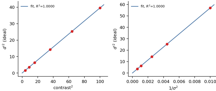
Figure 3. The transfer laws recovered from swept data. Left: ideal-observer d'^2 against contrast 2 , with the through-origin fit (coefficient of determination 1.000). Right: ideal-observer d'^2 against inverse noise variance 1/\sigma^2 , with the through-origin fit (coefficient of determination 1.000).
