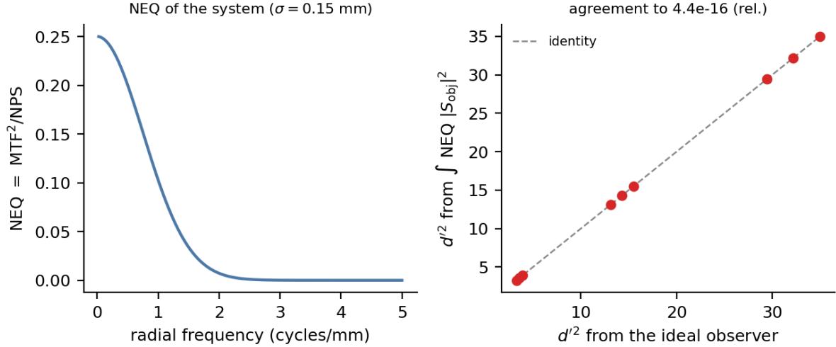
Figure 2: The physical-to-task bridge. Left: the \text{NEQ} = \text{MTF}^2/\text{NPS} of the system. Right: d'^2 computed from the ideal observer (horizontal) against d'^2 computed by integrating NEQ against the object power spectrum (vertical), for nine contrast-by-blur conditions; the points lie on the identity line to machine precision.
