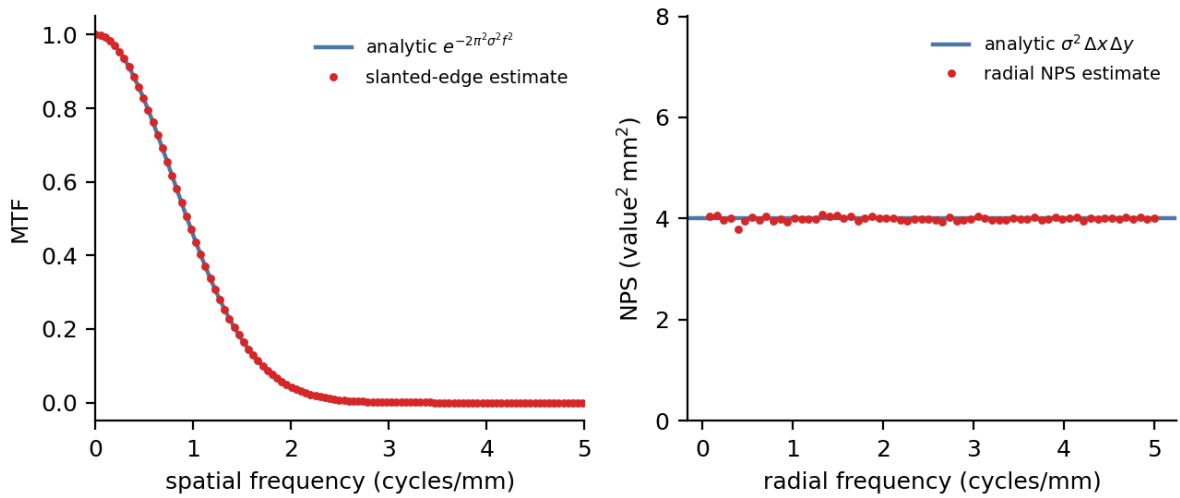
Figure 1: Physical estimators held to their closed forms. Left: the slanted-edge MTF estimate (points) against the analytic Gaussian \exp(-2\pi^2\sigma^2 f^2) (line) for an edge of blur 0.2 mm. Right: the radially averaged NPS estimate (points) against the analytic white level \sigma^2 dx dy (line) for noise of standard deviation 20 units.
