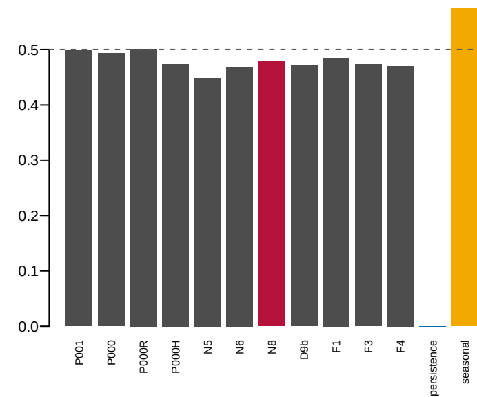
directional accuracy
