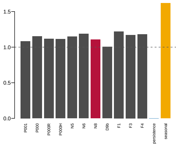
sd(pred)/sd(obs) (0 = flat)
