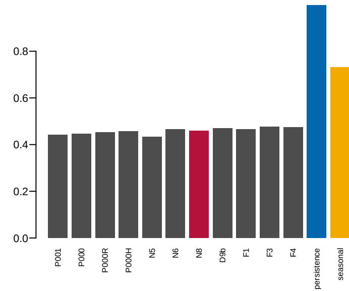
bias (1 = unbiased)
