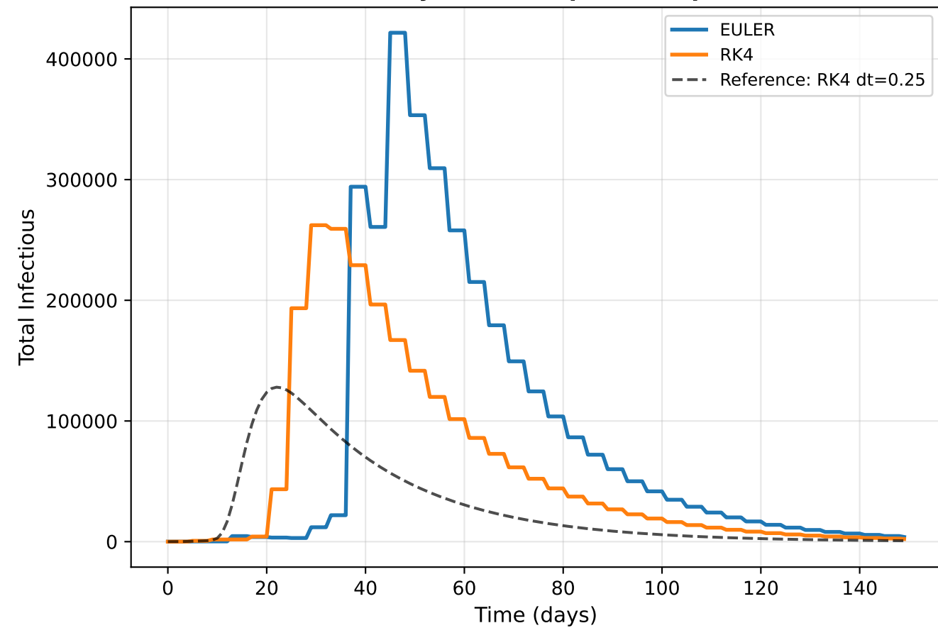
dt = 4.0 days (0.75 steps/latent period!)
