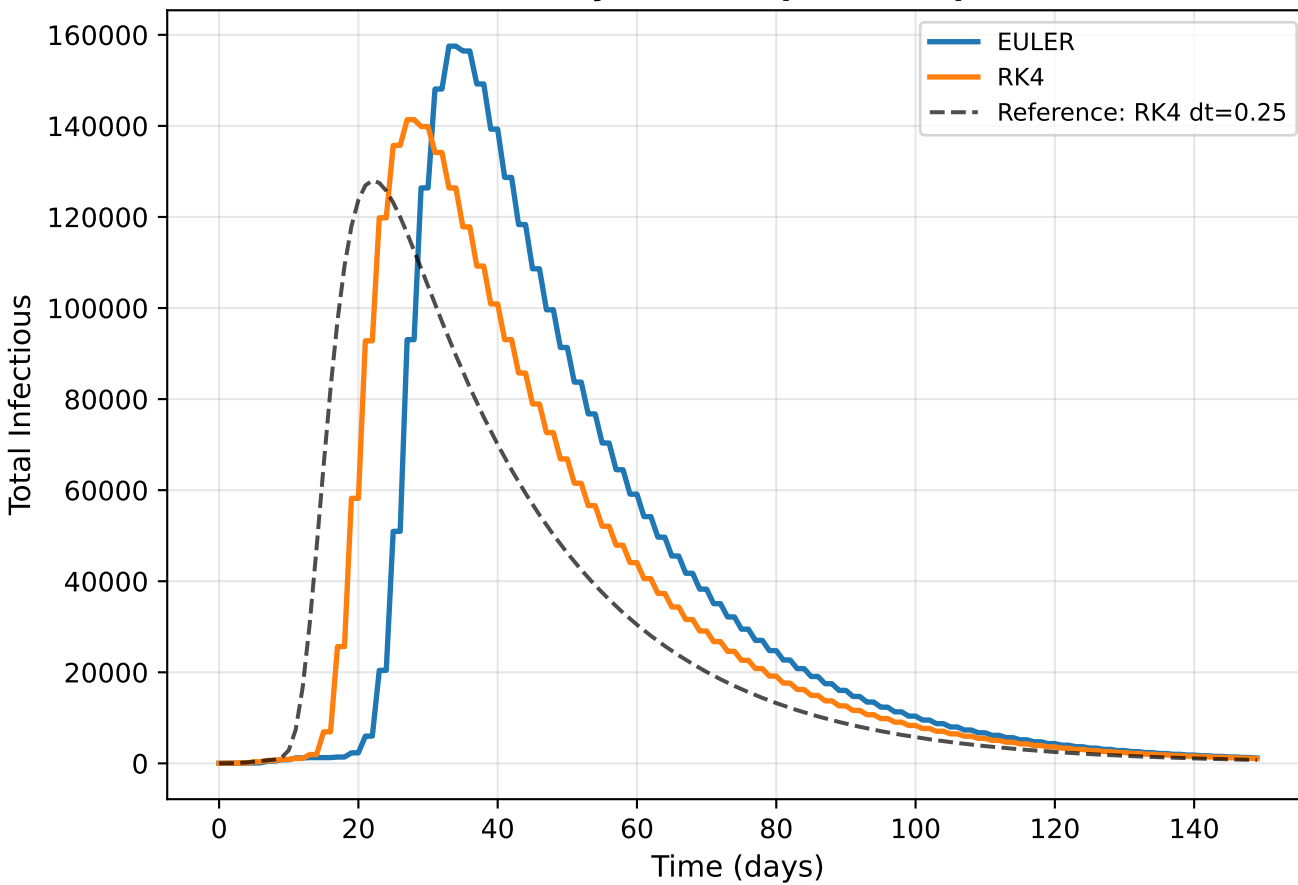
dt = 2.0 days (1.5 steps/latent period)
