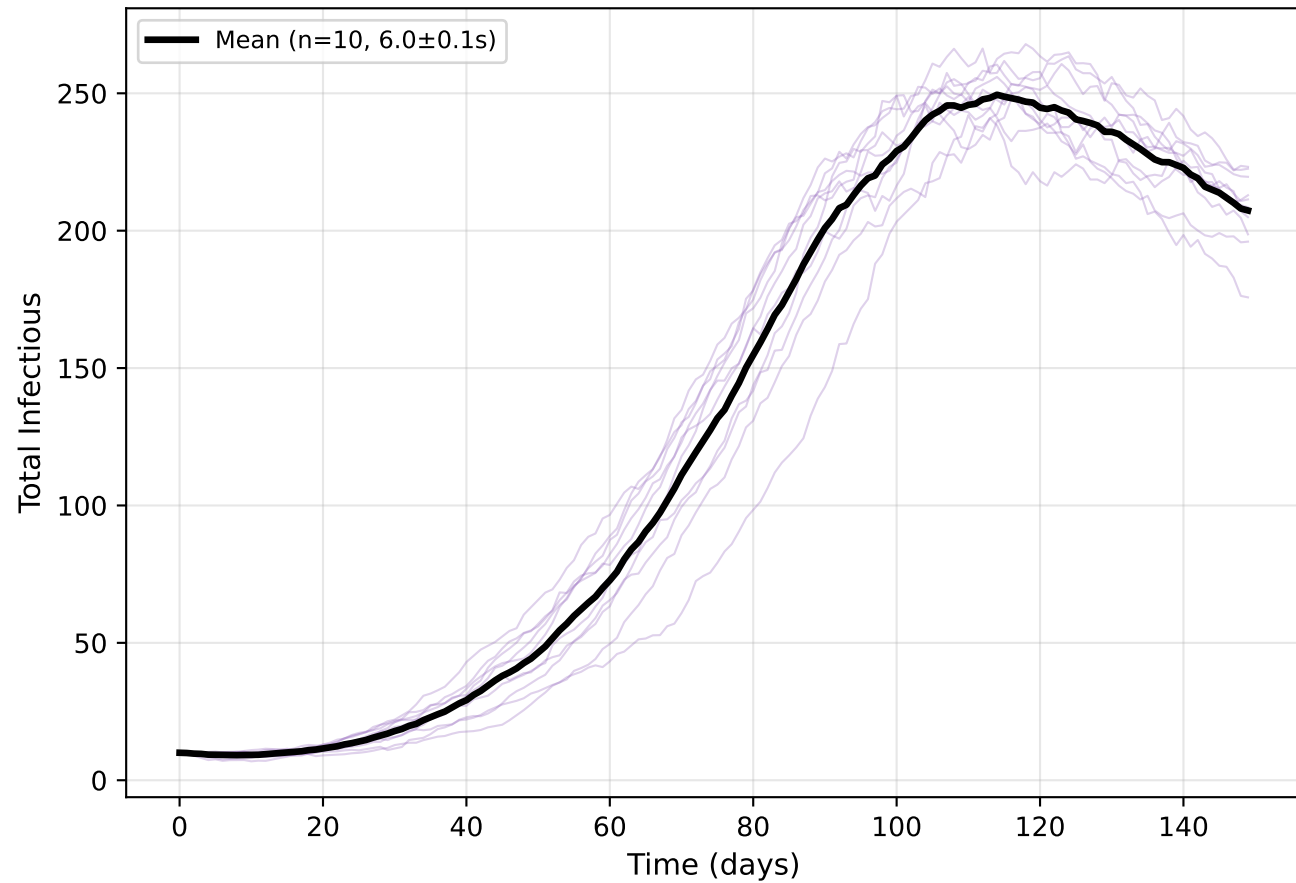
Hybrid (threshold=500)
