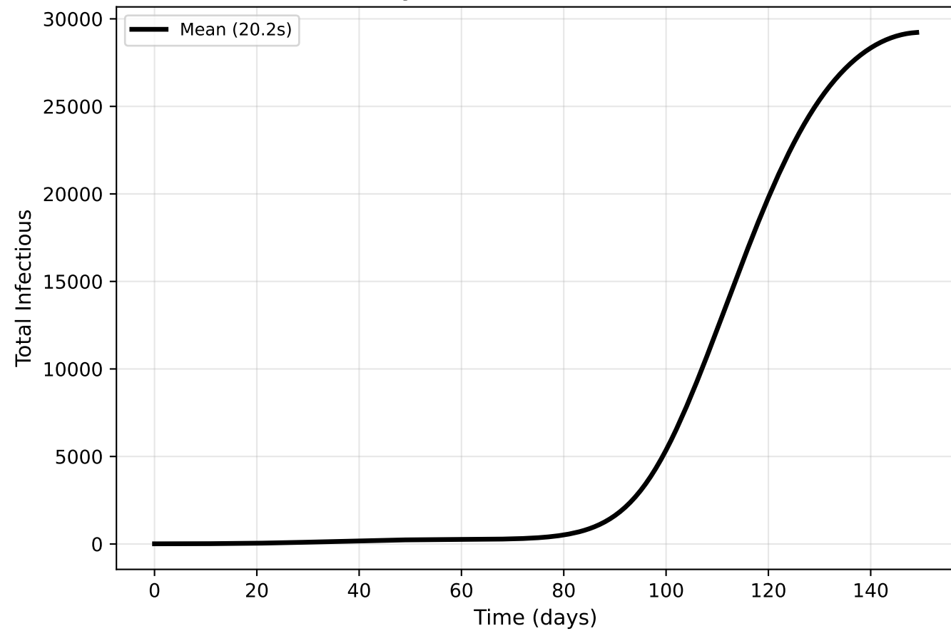
Hybrid (threshold=500)
