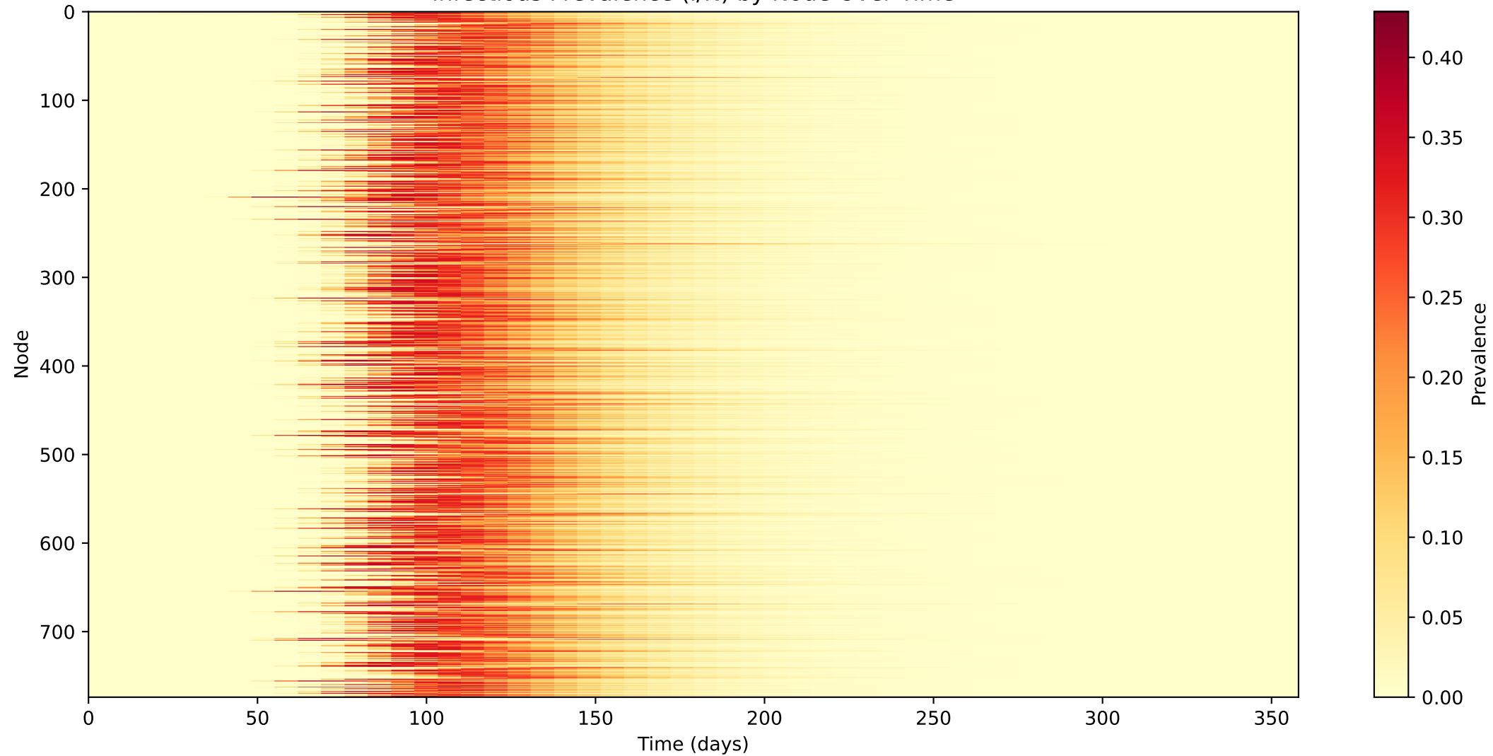
Infectious Prevalence (I/N) by Node Over Time
