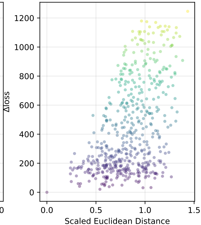
Δloss vs Distance from MLE
