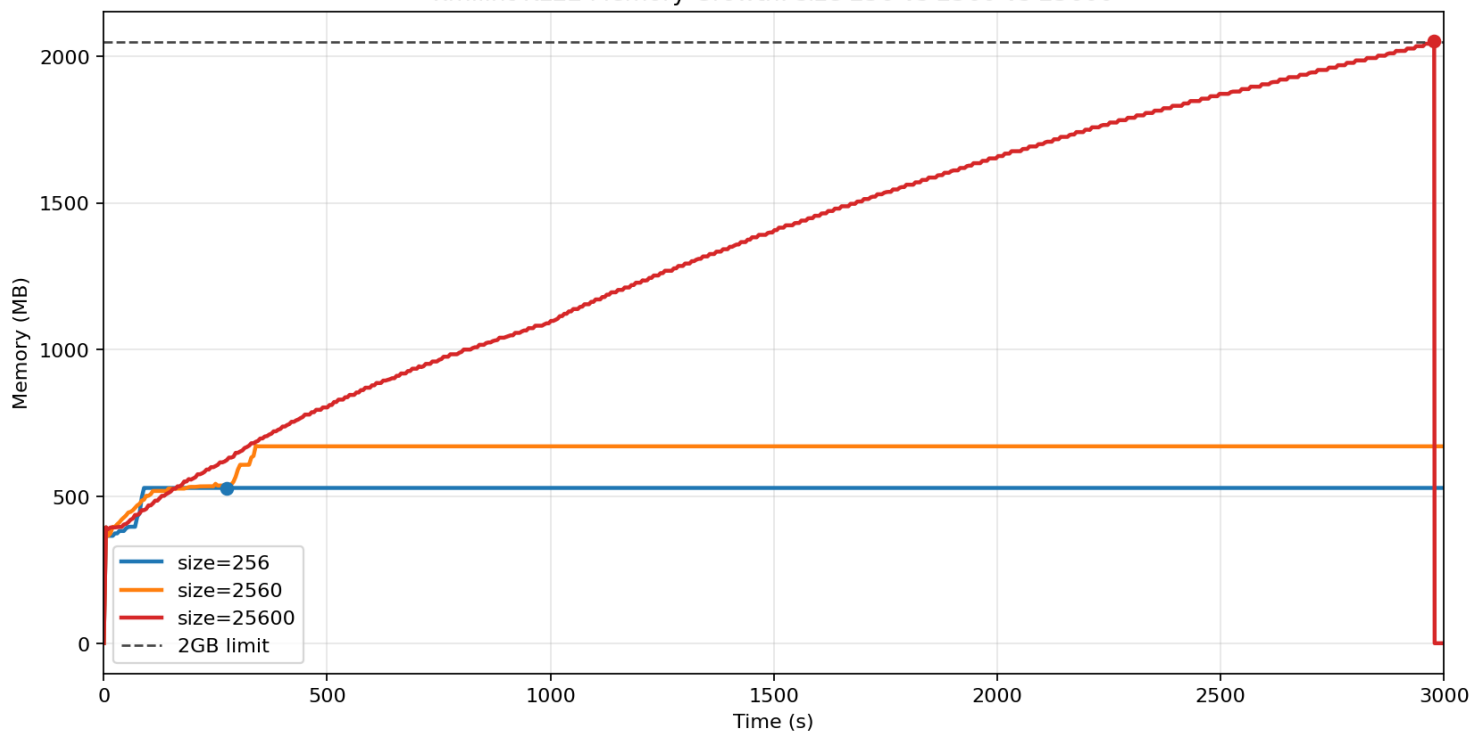
xmlint KLEE Memory Growth: size 256 vs 2560 vs 25600
