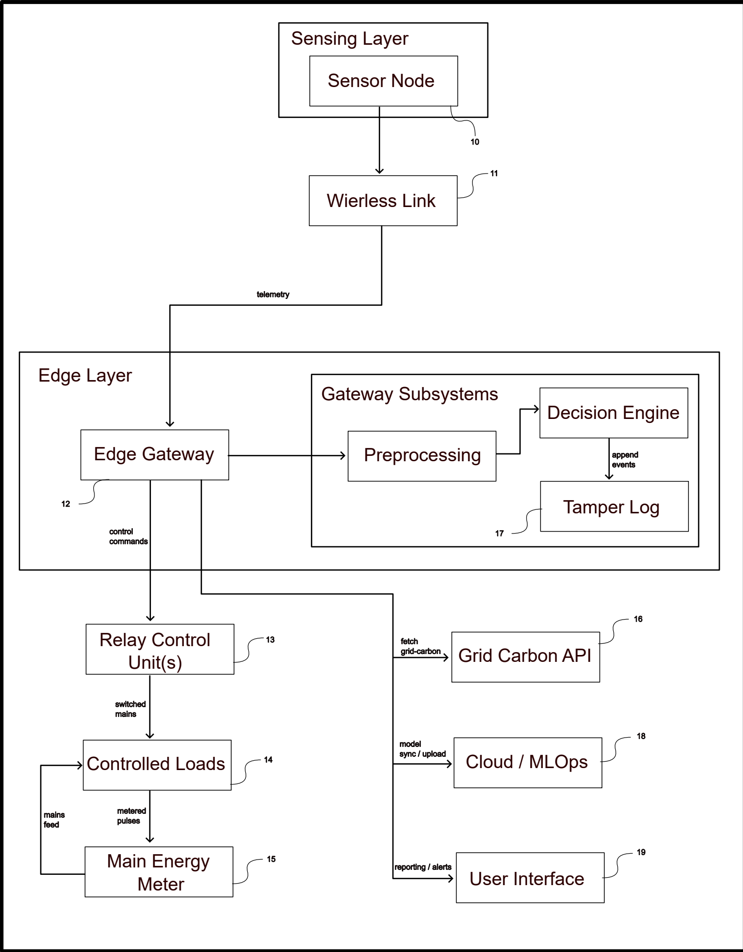
FIG. 1 System Architecture
