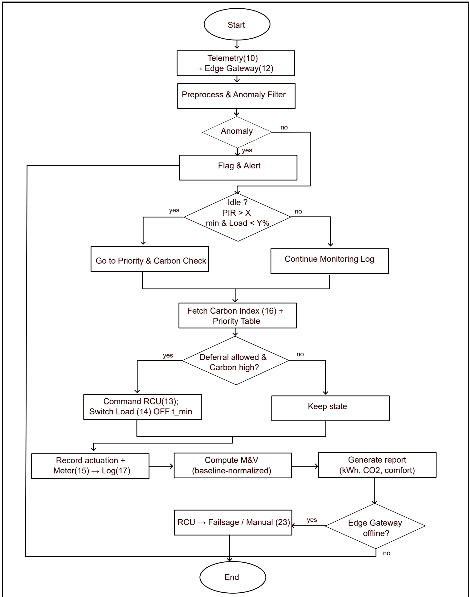
FIG. 3 Flow Control & M&V Sequence
