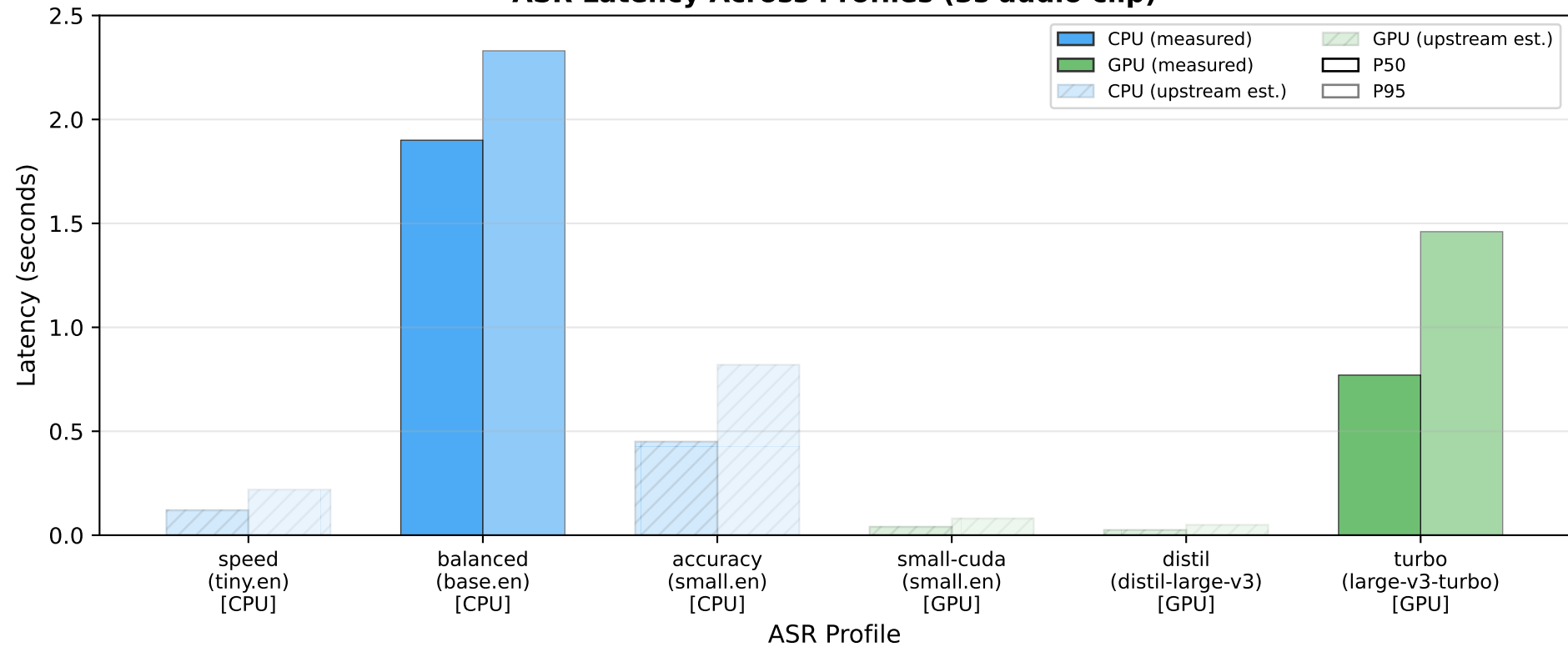
ASR Latency Across Profiles (3s audio clip)
