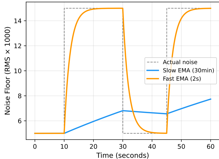
Dual-Timescale Noise Tracking
