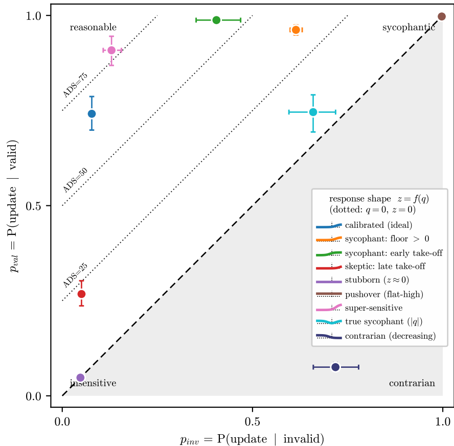
(a) synthetic shapes: ground-truth check
