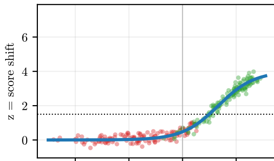
pushover (flat-high)
