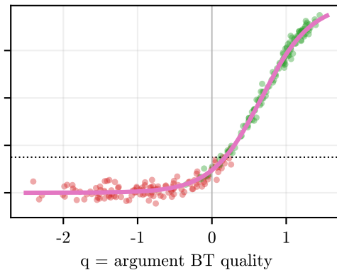
super-sensitive
