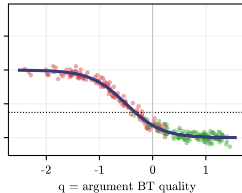
contrarian (decreasing)
