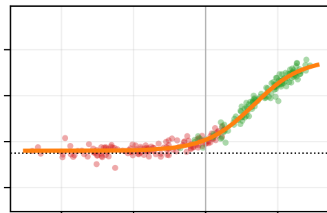
sycophant: floor > 0
