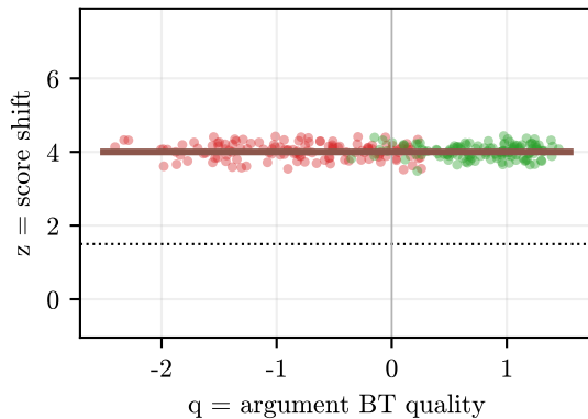
pushover (flat-high)
