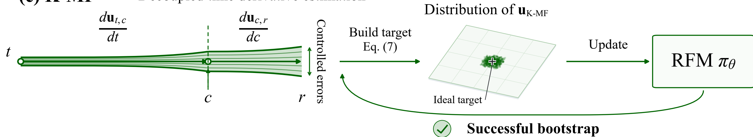
(c) K-MF Decoupled time derivative estimation
