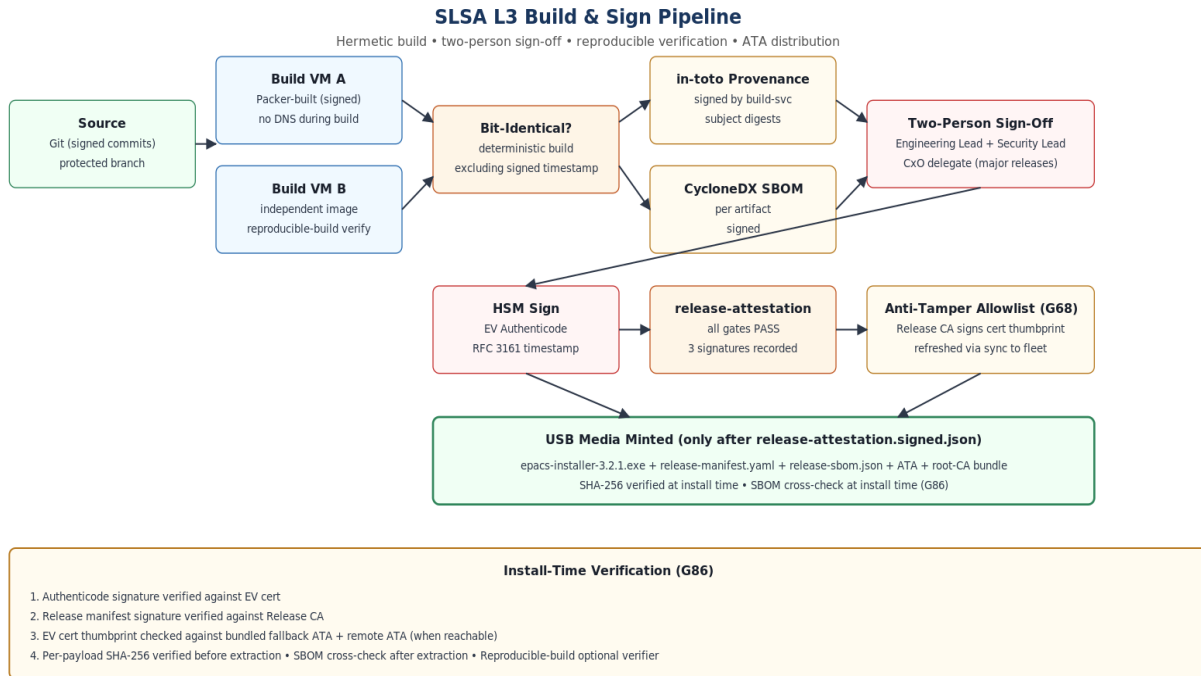
Figure: SLSA L3 Build & Sign Pipeline with ATA Distribution
