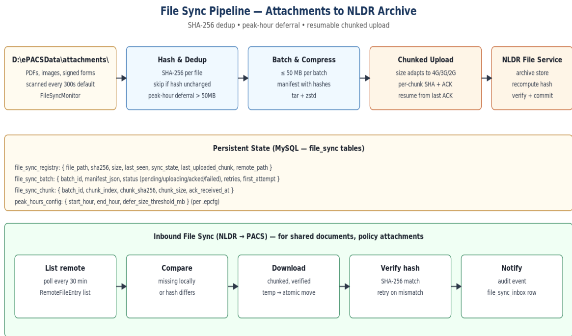
Figure: File Sync Pipeline — Hash Dedup, Peak-Hour Deferral, Resumable Chunked Upload
