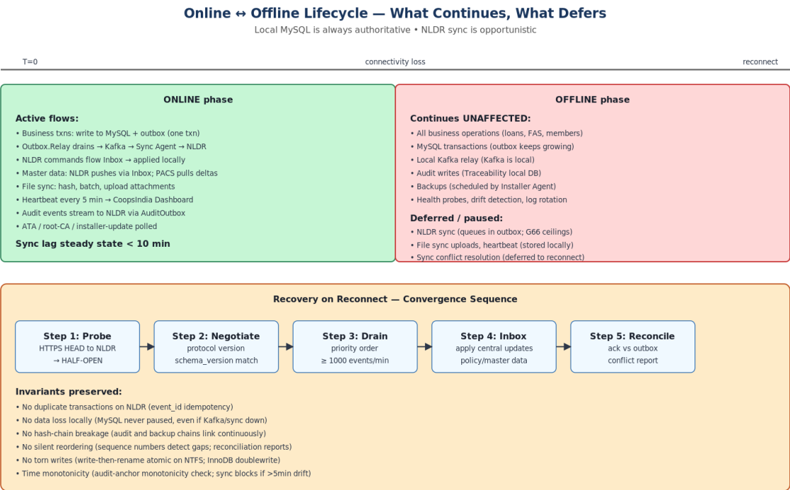
Figure: Online ↔ Offline Lifecycle — What Continues, What Defers, How Convergence Happens
