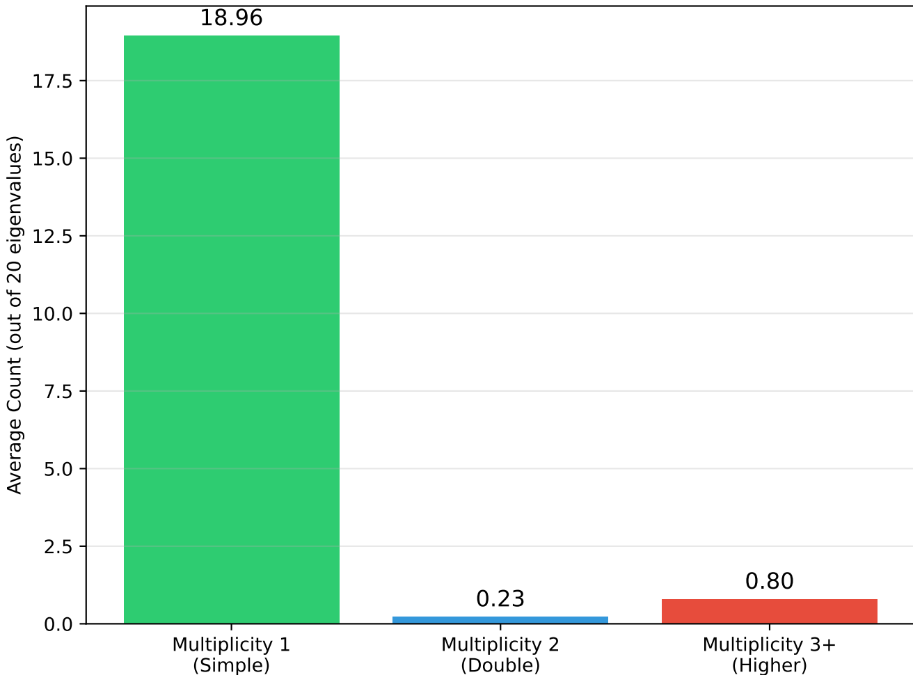
ModelNet40: Eigenvalue Multiplicity Distribution
