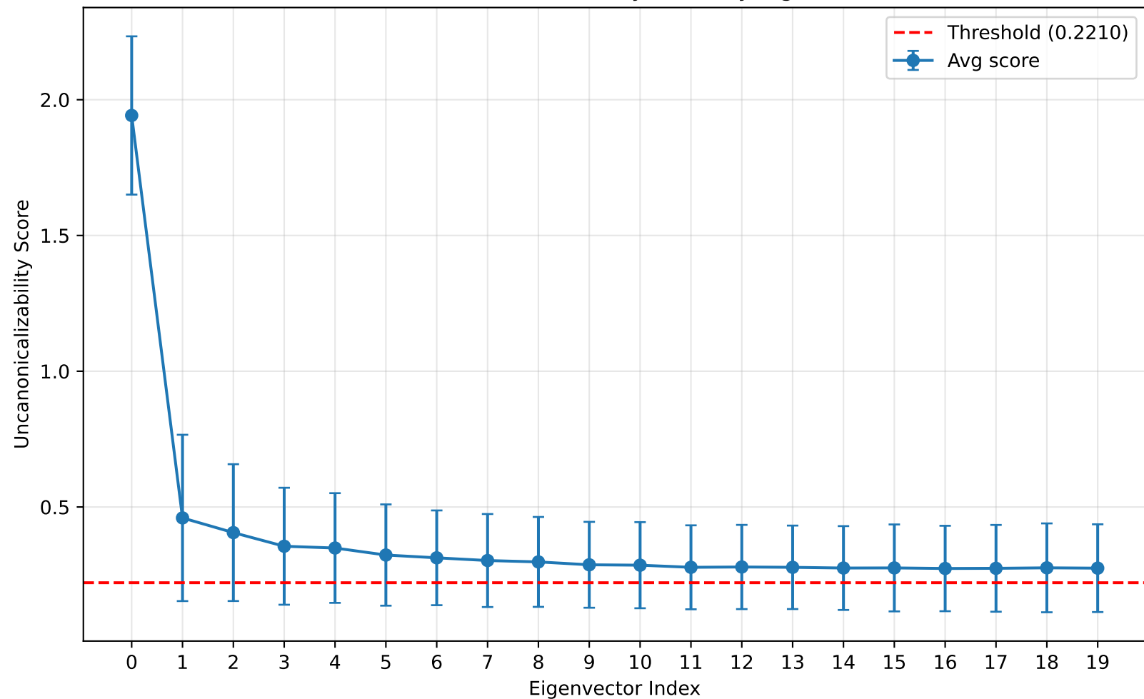
ModelNet40: Uncanonicalizability Score by Eigenvector Index
