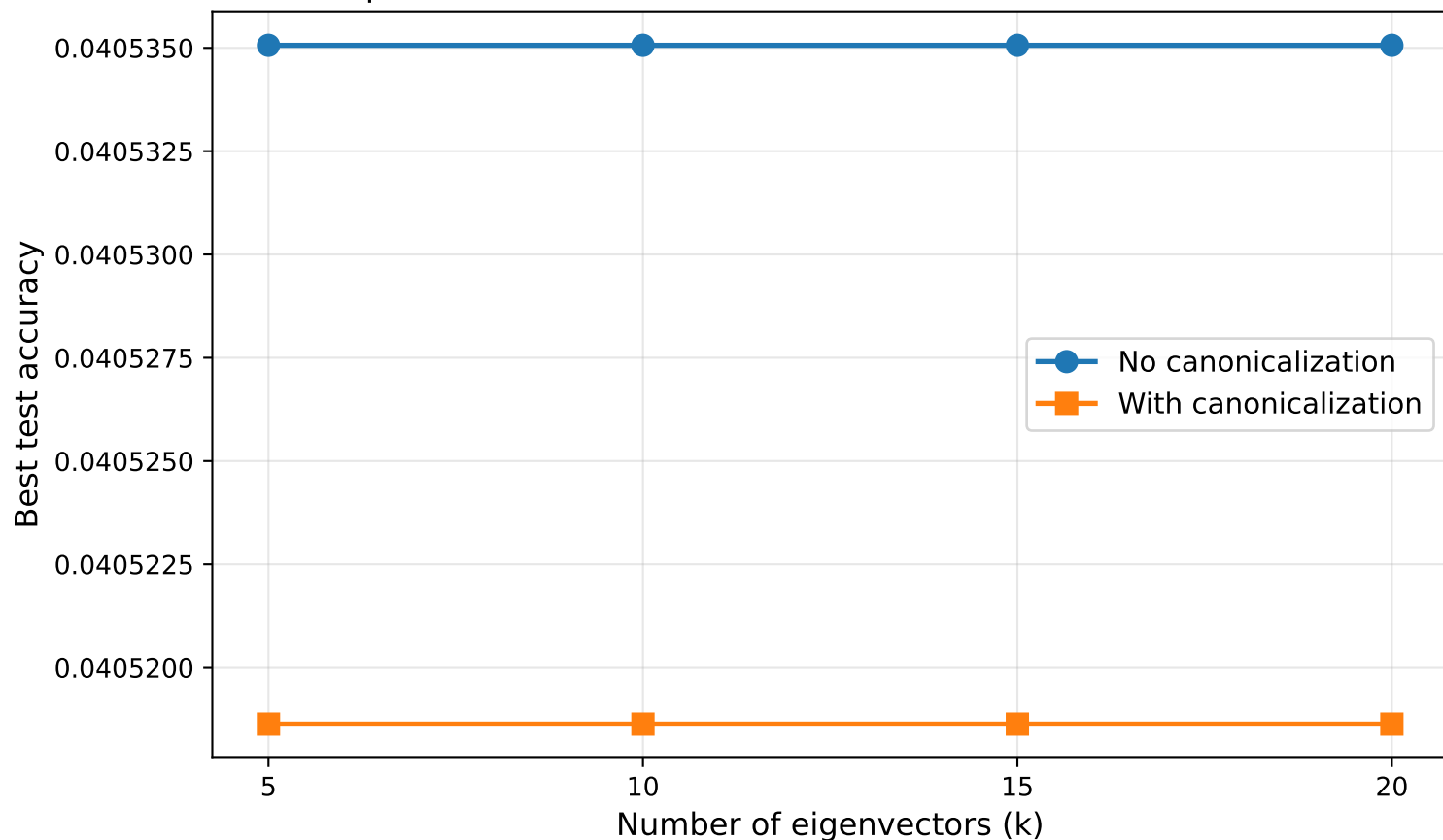
Spectral Transformer on ModelNet40: Canon vs No-Canon
