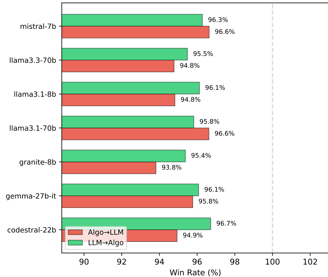
Wordle
