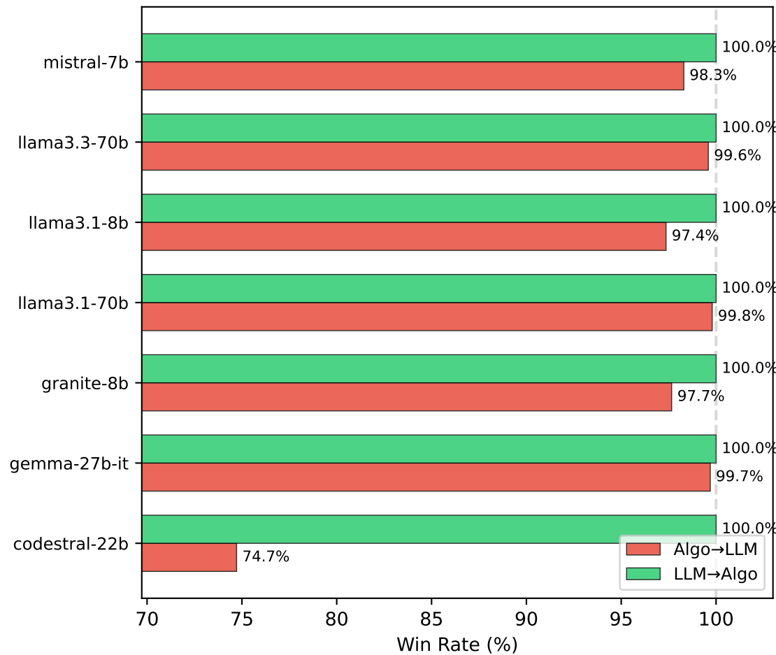
Mastermind Classic
