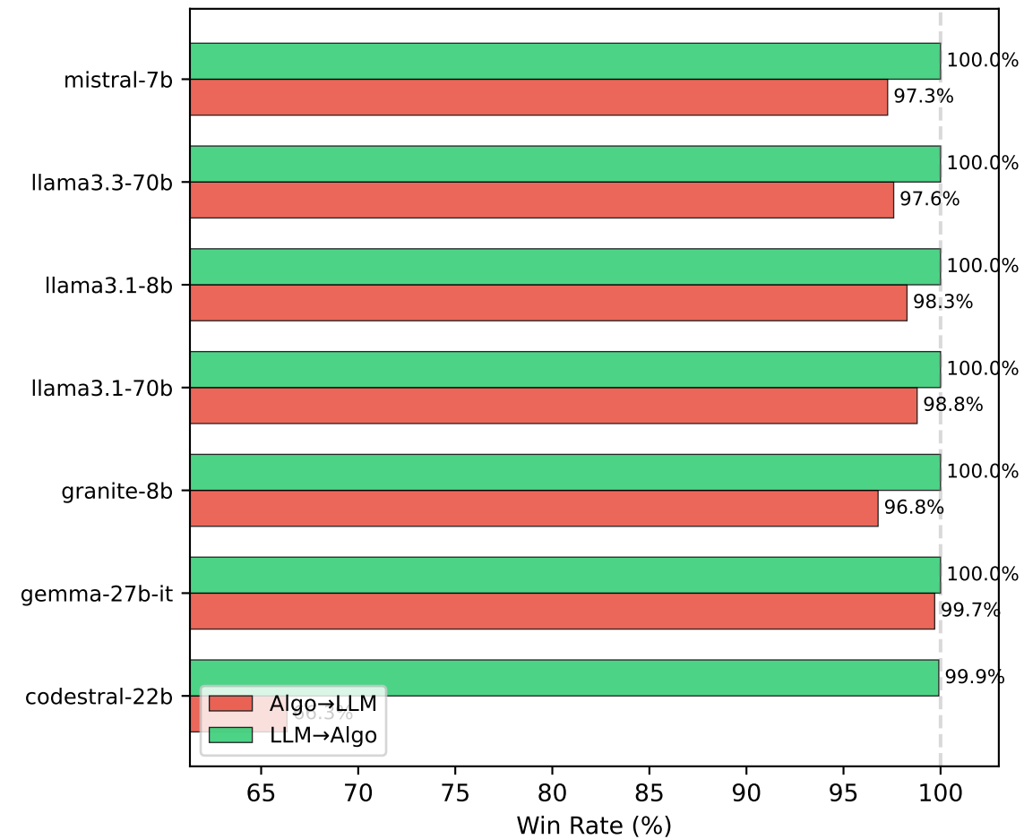
Mastermind Extended
